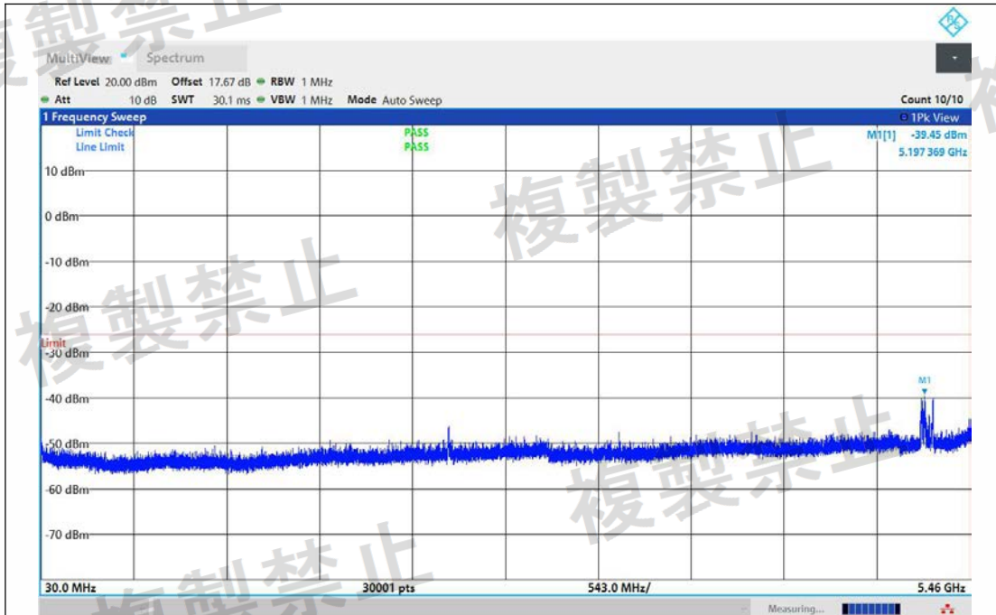
NTNV-11AX20MIMO-Ant1-5500-30~5460-PASS
