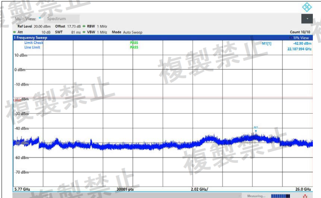
NTNV-11AX80MIMO-Ant1-5530-5770~26000-PASS
