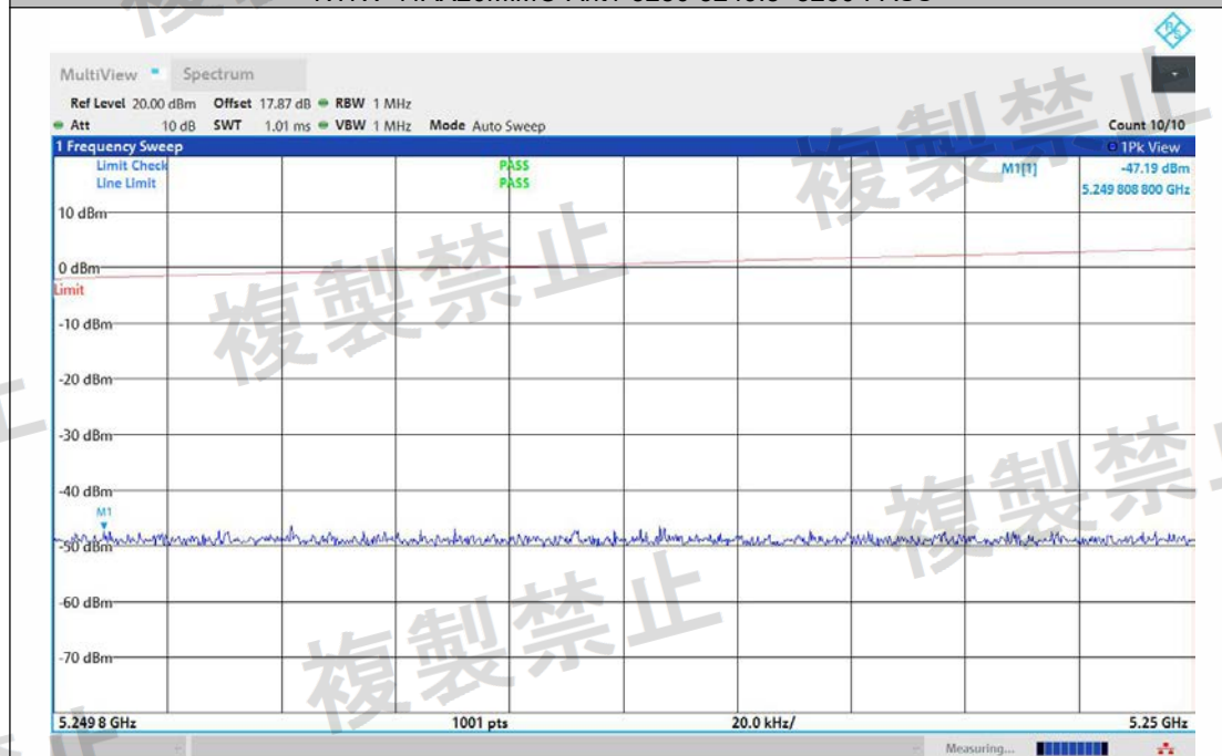
NTNV-11AX20MIMO-Ant2-5280-5249.8~5250-PASS
