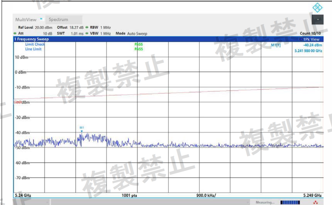
NTNV-11AX20MIMO-Ant2-5320-5240~5249-PASS
