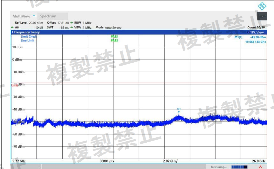
NTVN-11AX40MIMO-Ant2-5510-5770~26000-PASS
