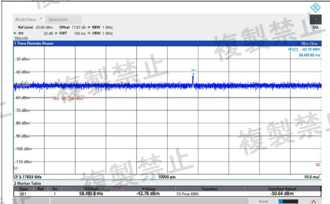
NTNV-11N20MIMO-Ant2-5280-30~5233.3-PASS
