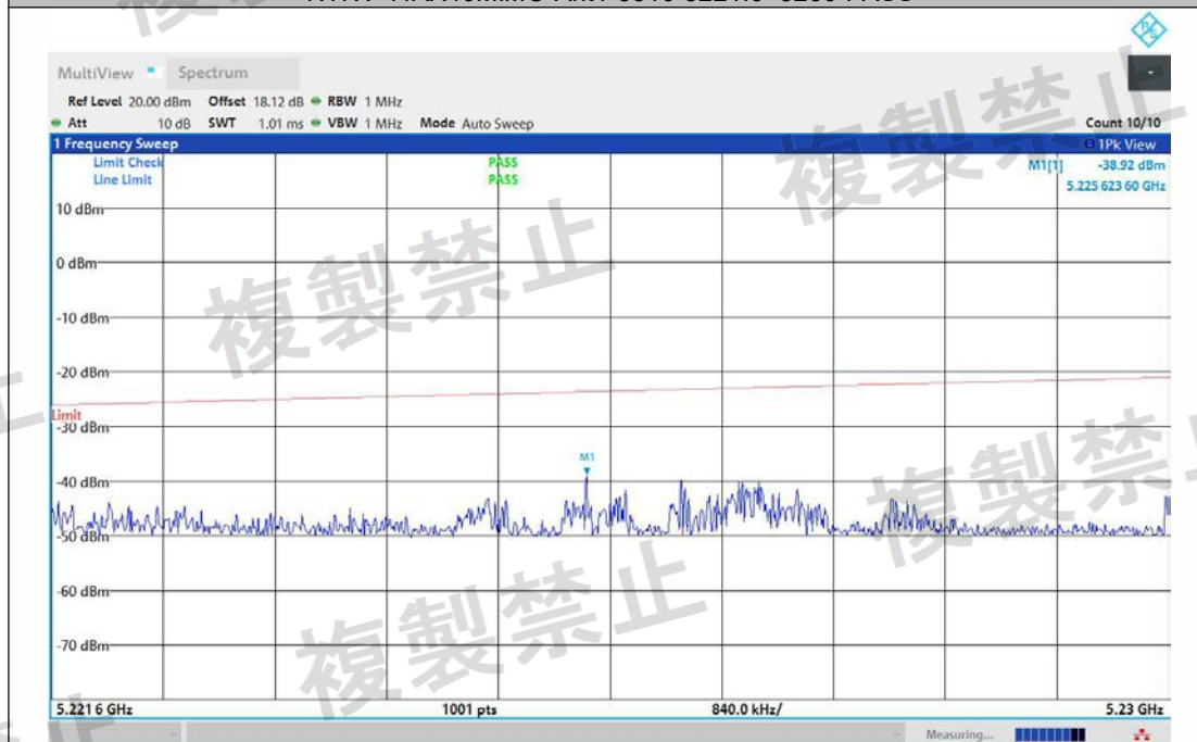
NTNV-11AX40MIMO-Ant2-5310-5221.6~5230-PASS
