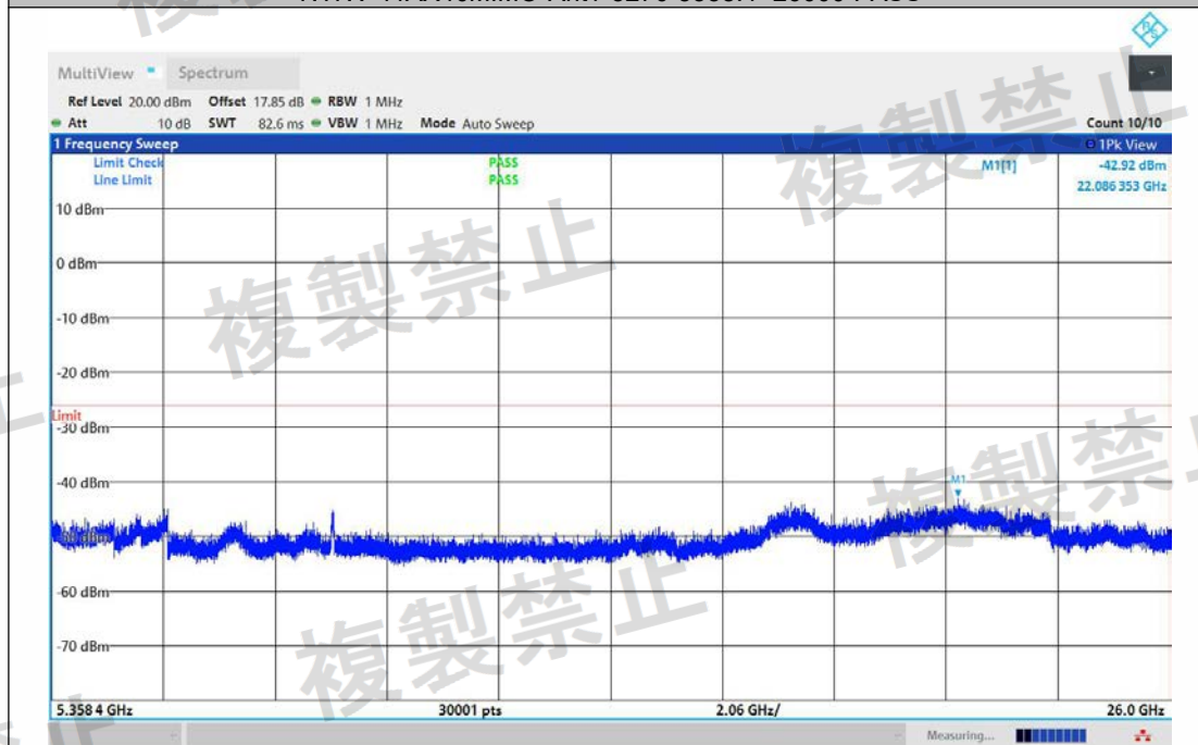
NTNV-11AX40MIMO-Ant2-5270-5358.4~26000-PASS
