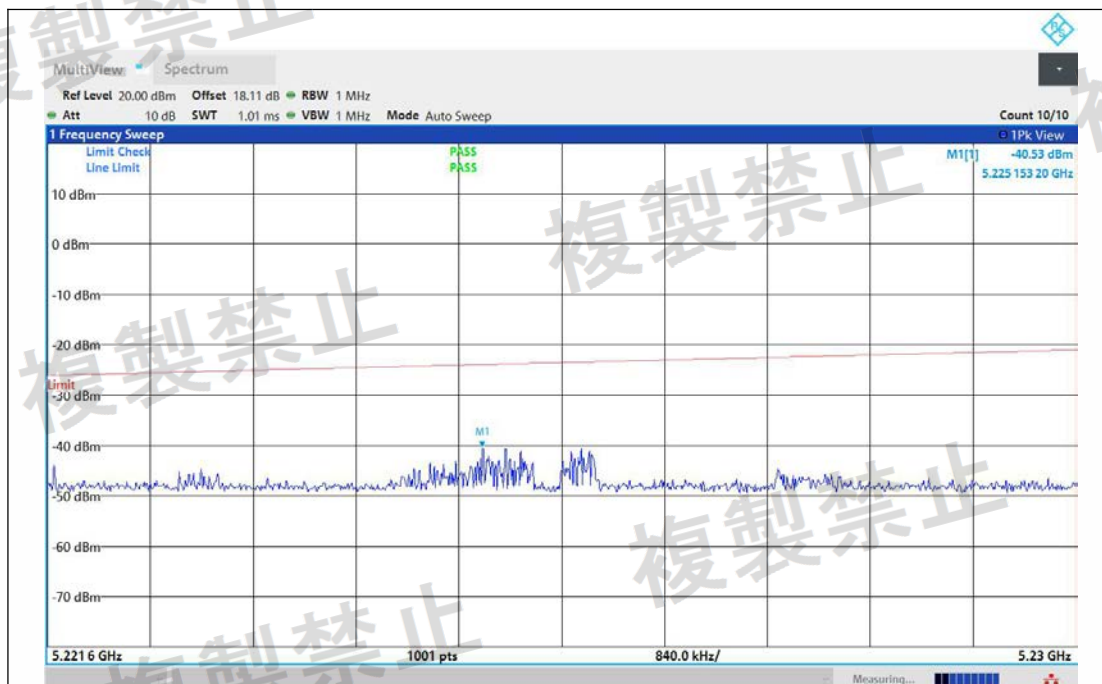
NTNV-11AX40MIMO-Ant1-5310-5221.6~5230-PASS
