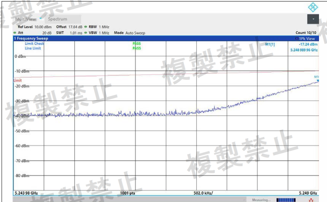
NTNV-11N20MIMO-Ant1-5260-5240~5249-PASS
