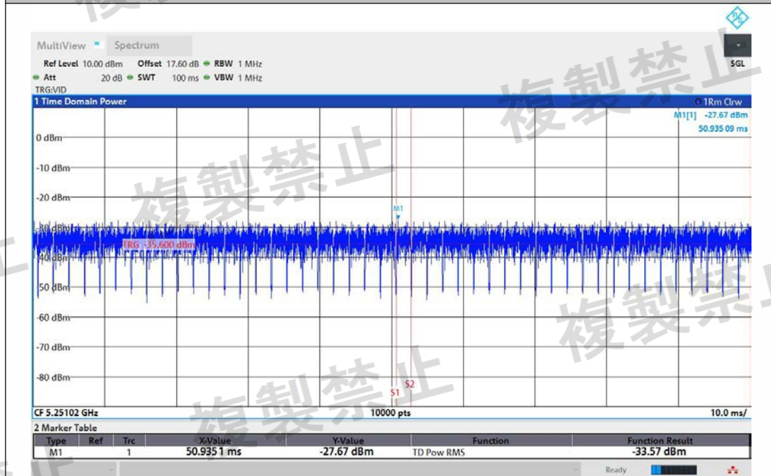
NTNV-11A-Ant2-5240-5251~5260-PASS
