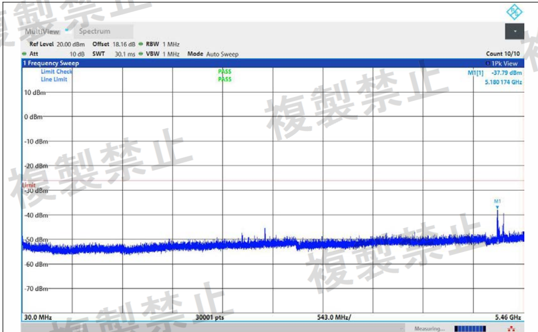
NTNV-11AX20MIMO-Ant1-5580-30~5460-PASS
