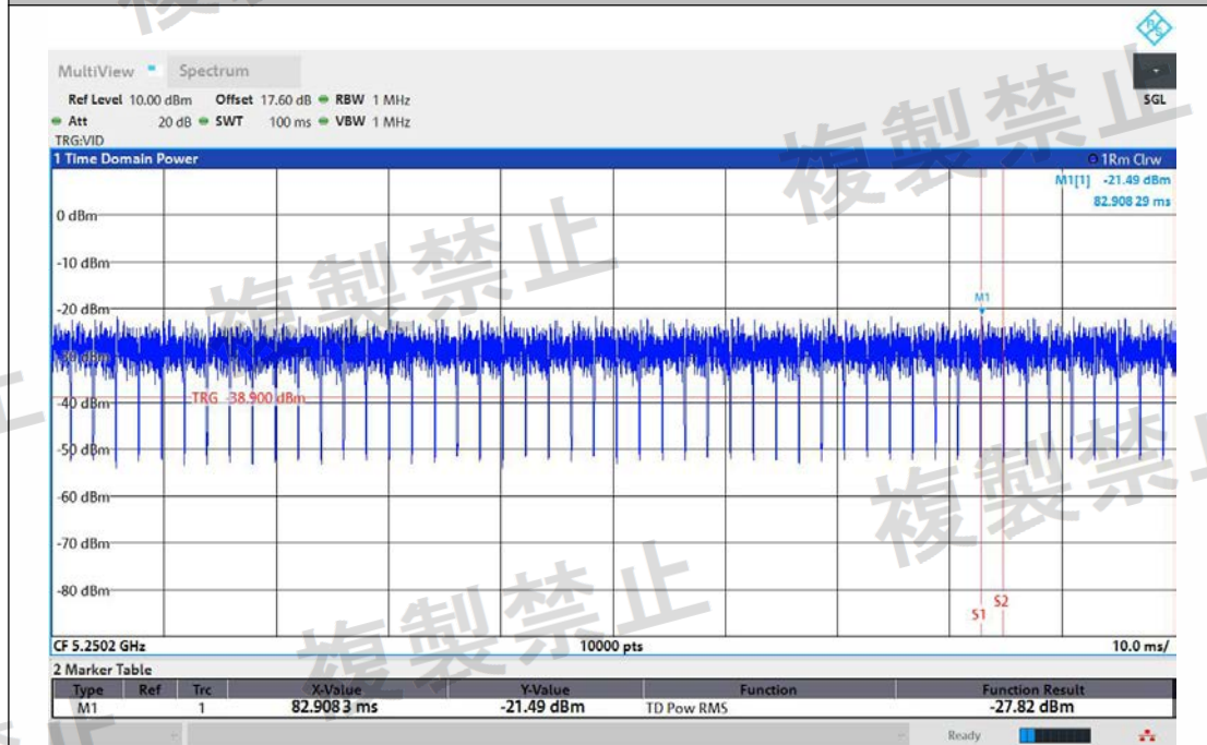
NTNV-11N20MIMO-Ant1-5240-5250~5250.2-PASS
