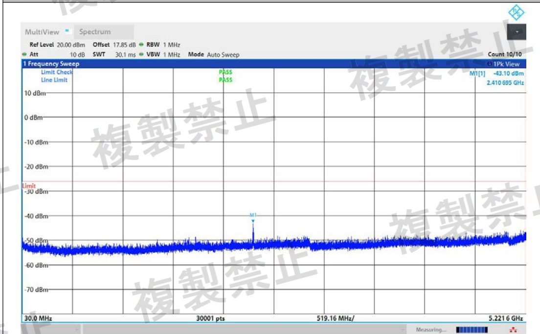
NTNV-11AX40MIMO-Ant2-5270-30~5221.6-PASS
