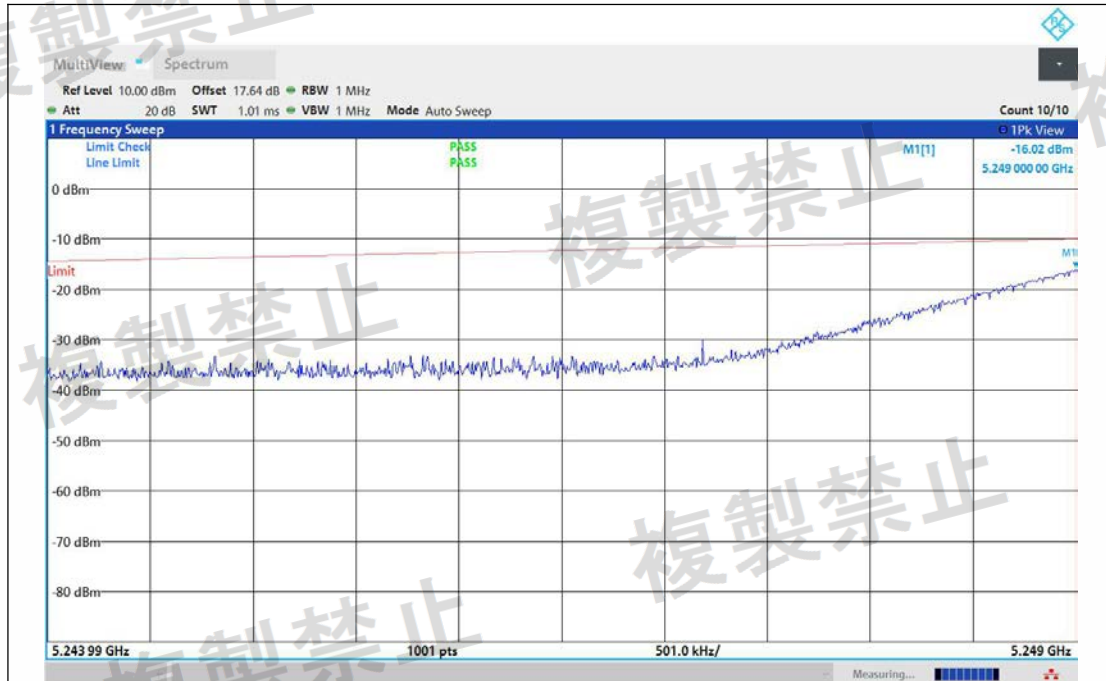
NTNV-11A-Ant1-5260-5240~5249-PASS
