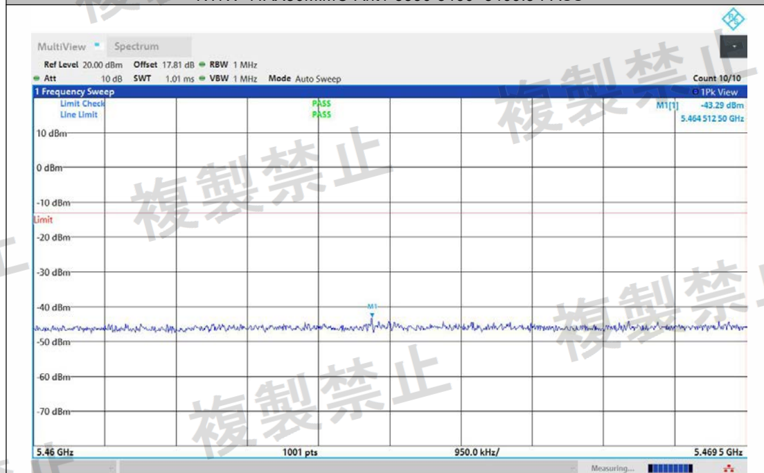
NTNV-11AX80MIMO-Ant2-5530-5460~5469.5-PASS
