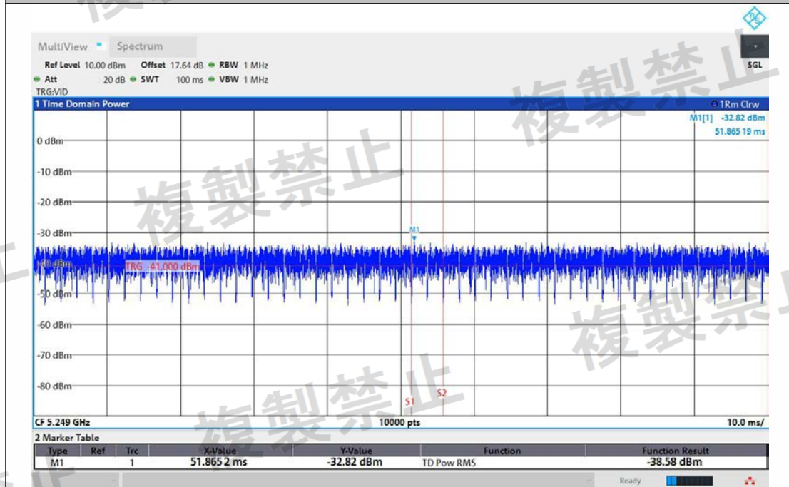
NTNV-11A-Ant1-5260-5240~5249-PASS
