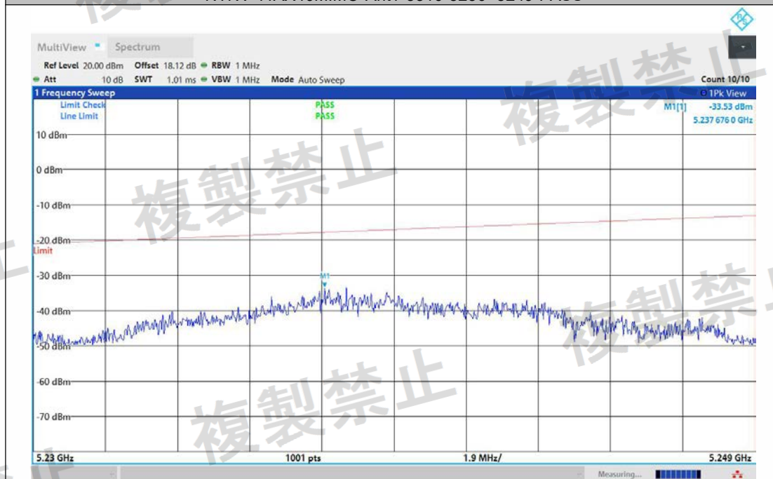
NTNV-11AX40MIMO-Ant2-5310-5230~5249-PASS
