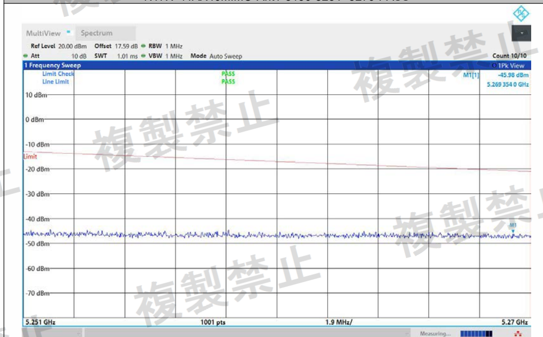
NTNV-11AX40MIMO-Ant2-5190-5251~5270-PASS
