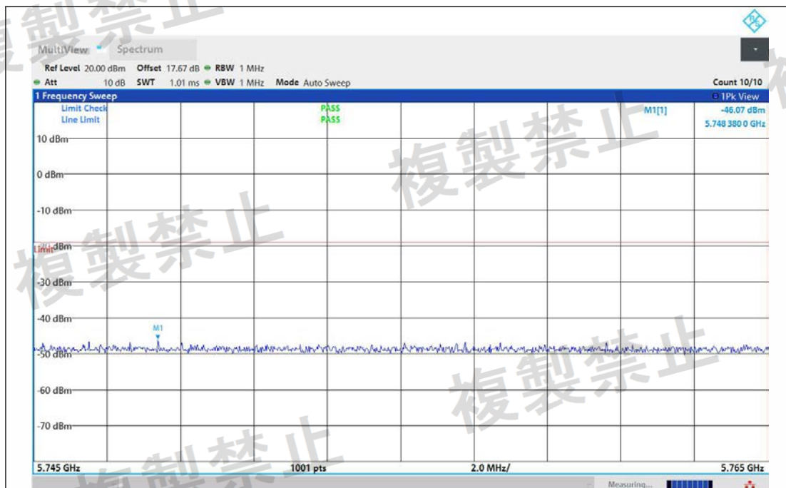
NTNV-11AX20MIMO-Ant1-5500-5745~5765-PASS
