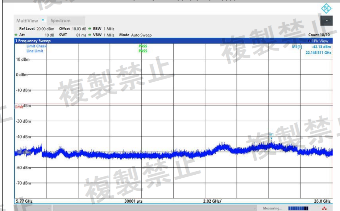
NTNV-11AX40MIMO-Ant2-5670-5770~26000-PASS
