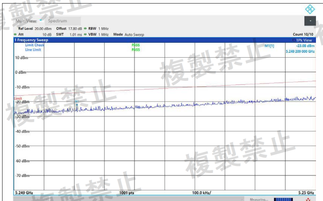
NTNV-11AX80MIMO-Ant1-5290-5249~5250-PASS
