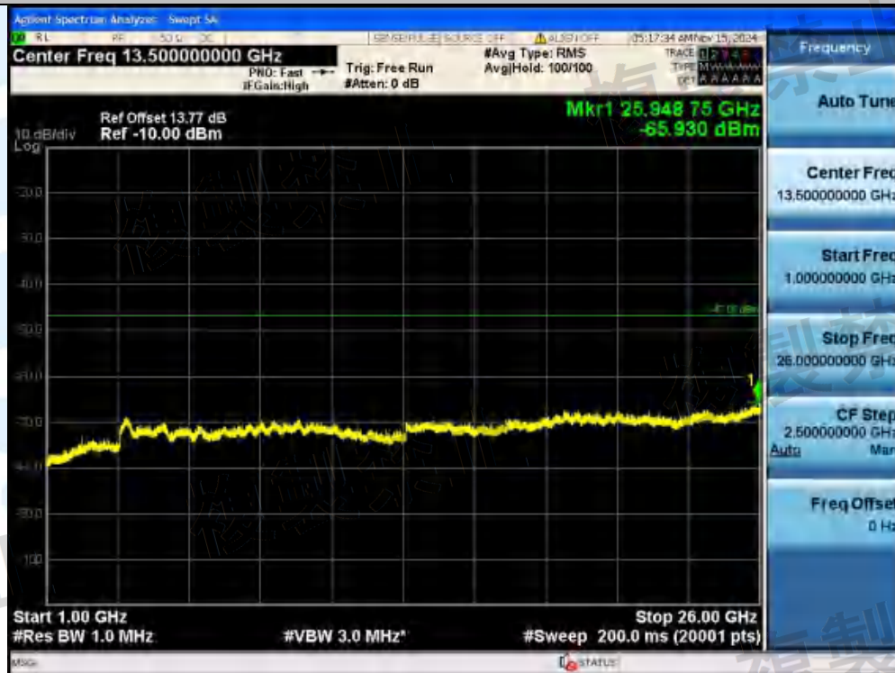
NTVN-11AX80MIMO-Ant2-5210-484Tone-RU65-1000~26000-PASS
