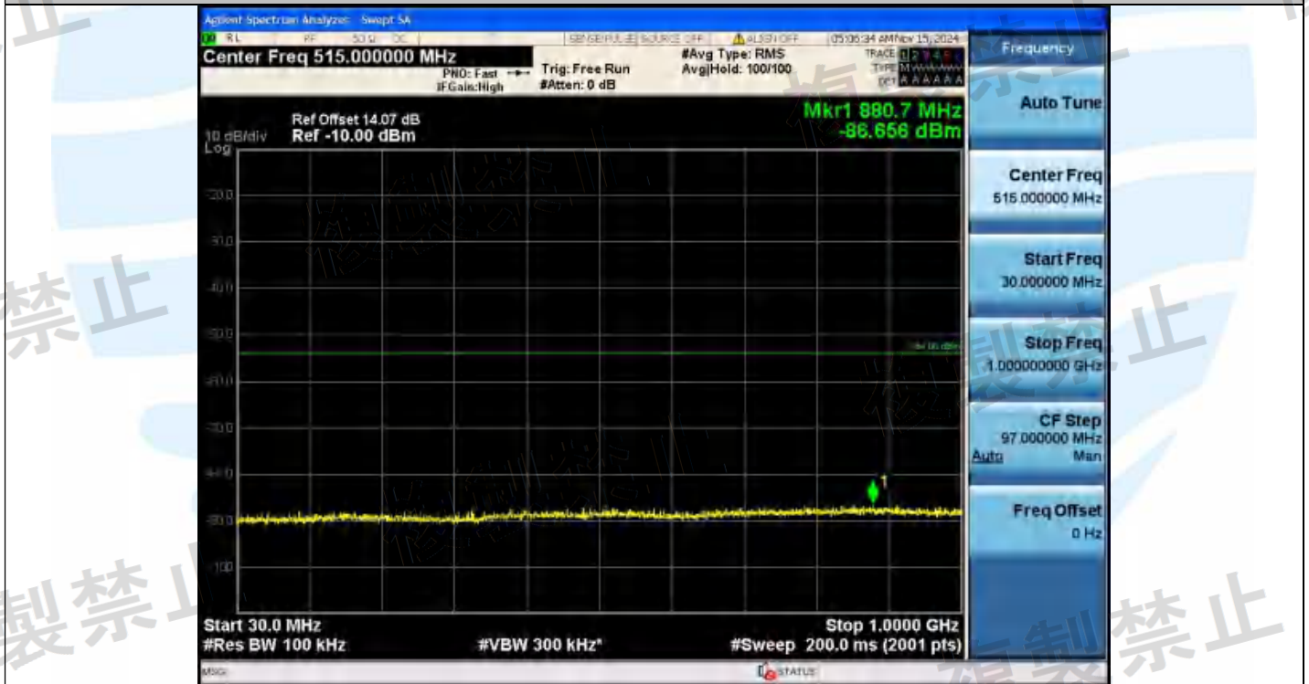
NTNV-11AX40MIMO-Ant2-5670-242Tone-RU61-30~1000-PASS
