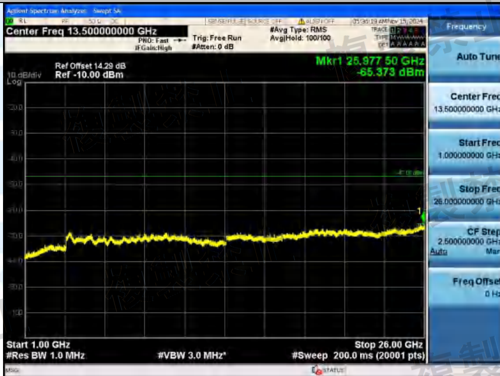
NTNV-11AX80MIMO-Ant2-5610-242Tone-RU64-1000~26000-PASS
