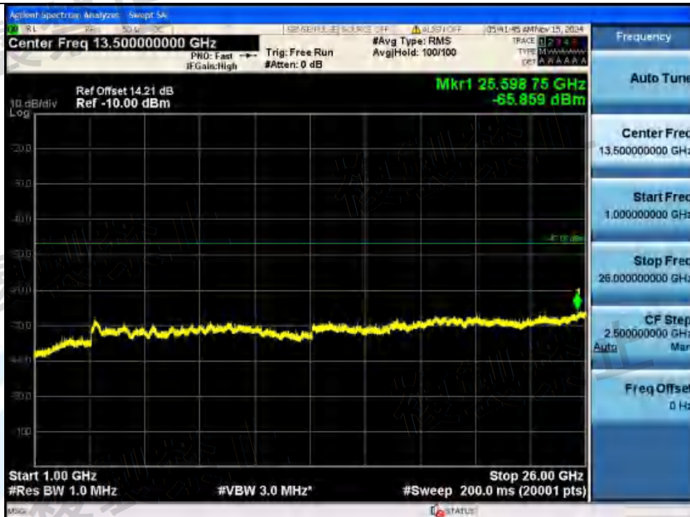
NTNV-11AX80MIMO-Ant1-5690-484Tone-RU65-1000~26000-PASS
