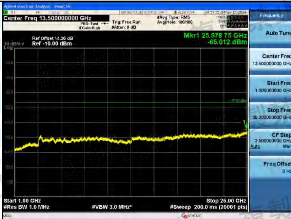
NTVN-11AX40MIMO-Ant2-5310-242Tone-RU62-1000~26000-PASS
