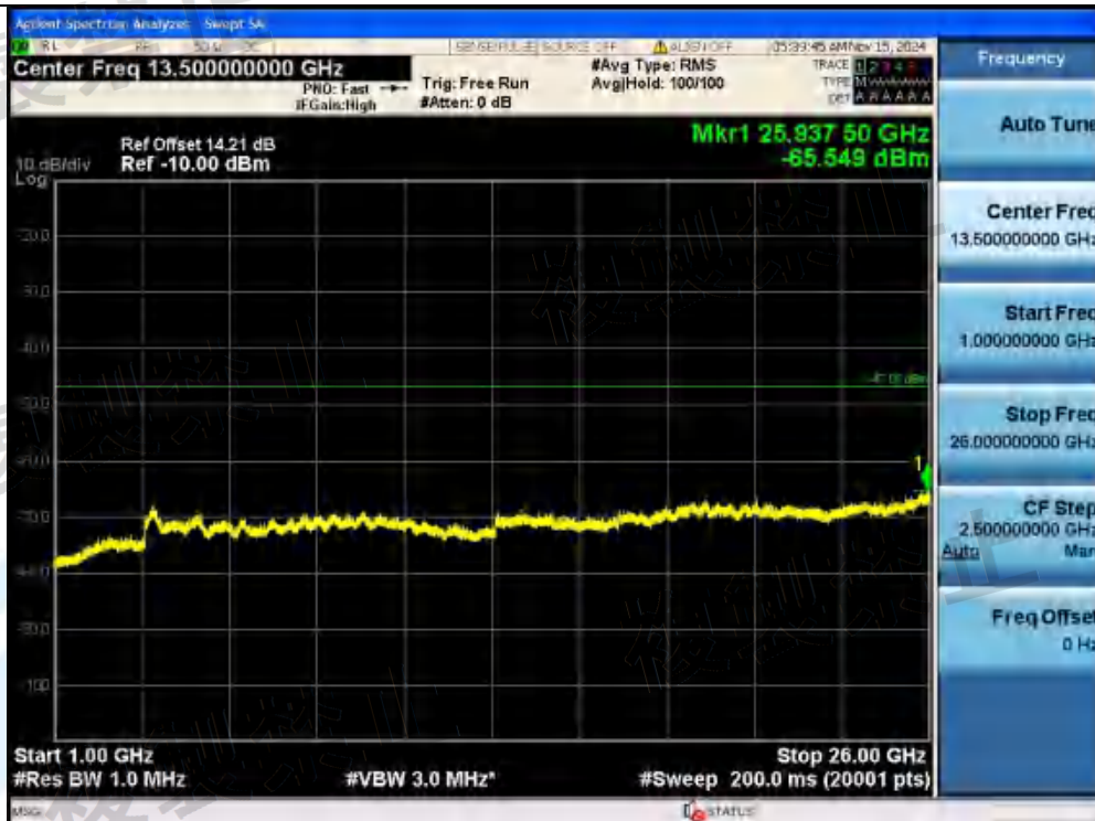
NTNV-11AX80MIMO-Ant1-5690-242Tone-RU61-1000~26000-PASS
