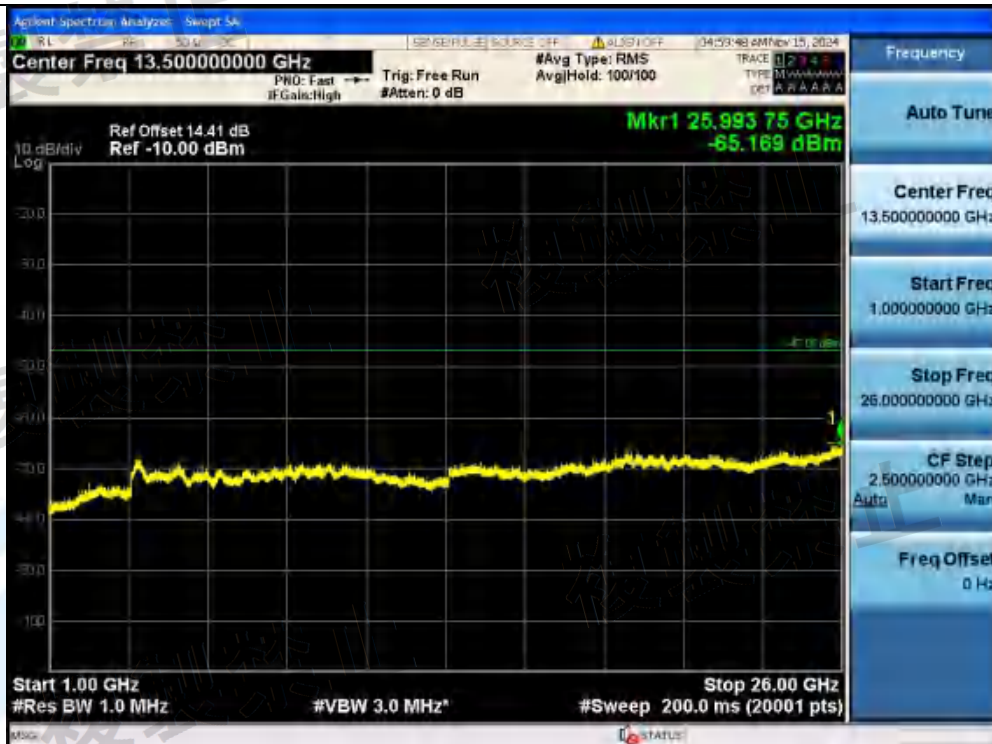
NTVN-11AX40MIMO-Ant1-5510-242Tone-RU61-1000~26000-PASS
