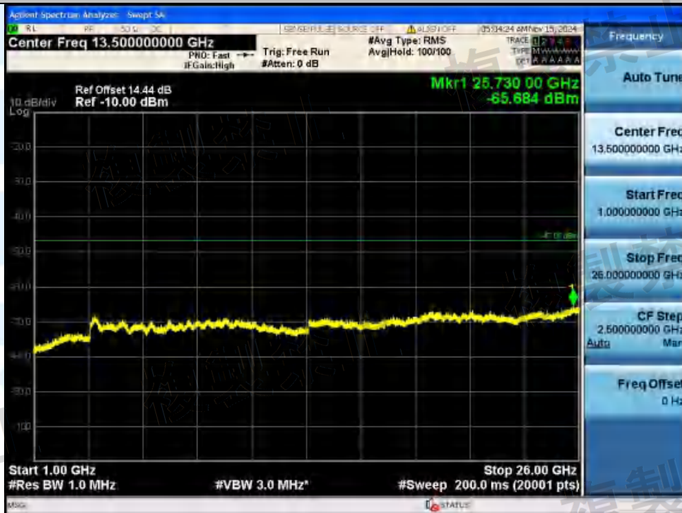
NTNV-11AX40MIMO-Ant2-5550-242Tone-RU62-1000~26000-PASS
