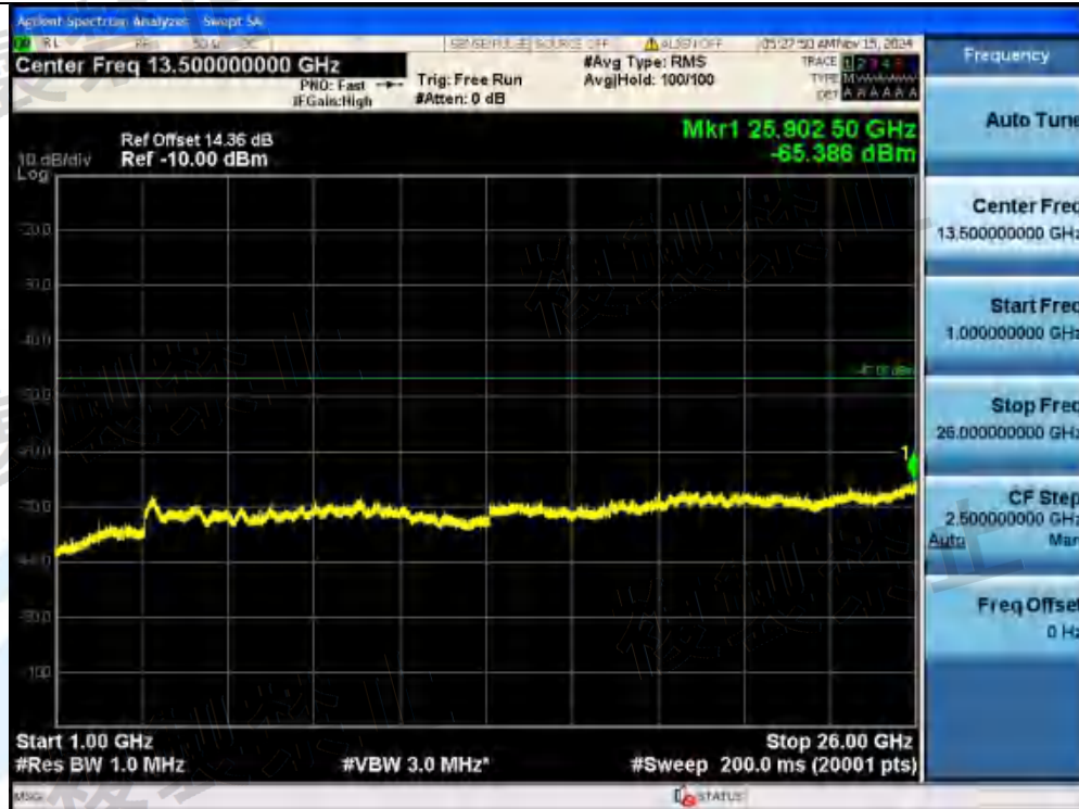
NTNV-11AX80MIMO-Ant1-5530-484Tone-RU65-1000~26000-PASS
