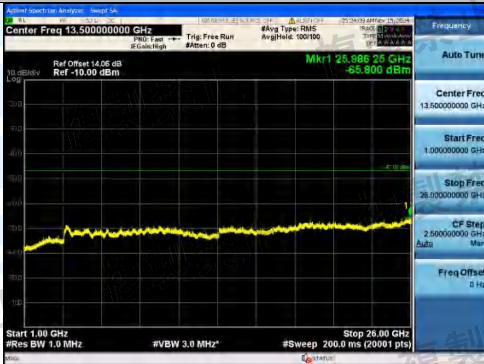
NTVN-11AX80MIMO-Ant2-5290-484Tone-RU66-1000~26000-PASS
