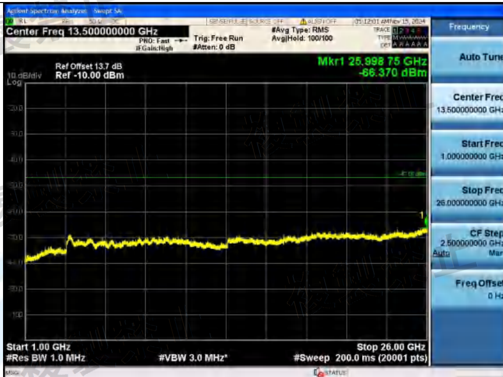
NTNV-11AX80MIMO-Ant1-5210-242Tone-RU61-1000~26000-PASS
