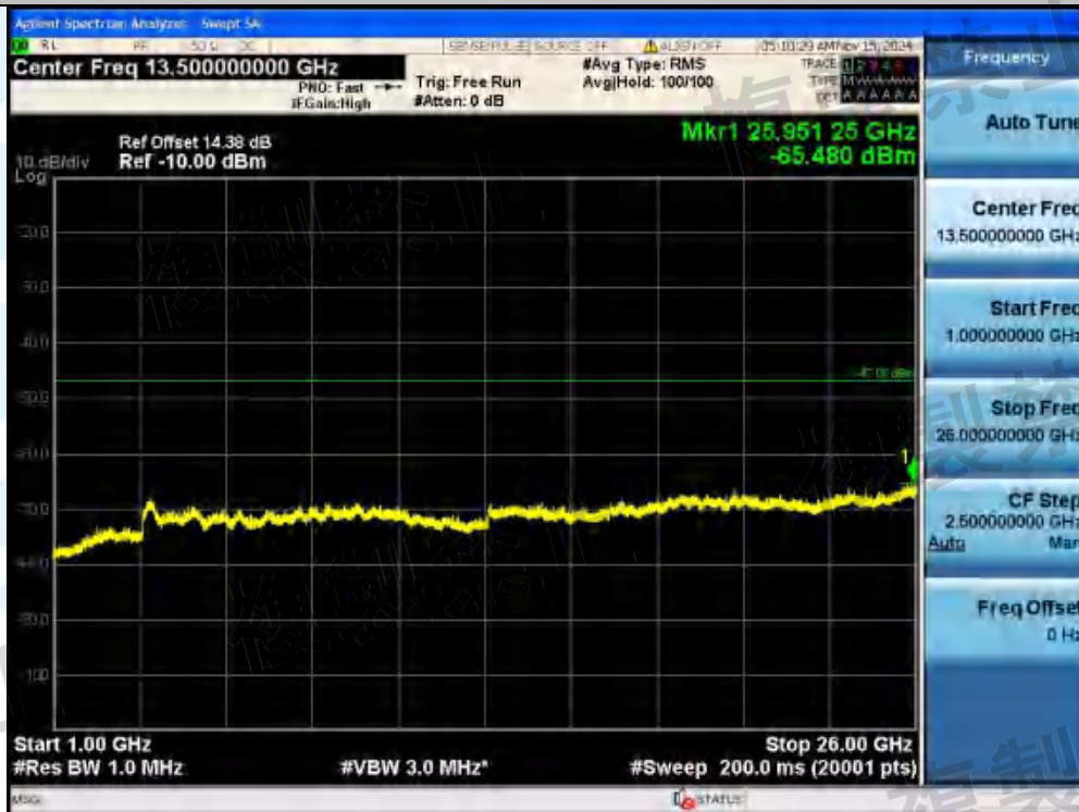
NTNV-11AX40MIMO-Ant2-5710-242Tone-RU62-1000~26000-PASS
