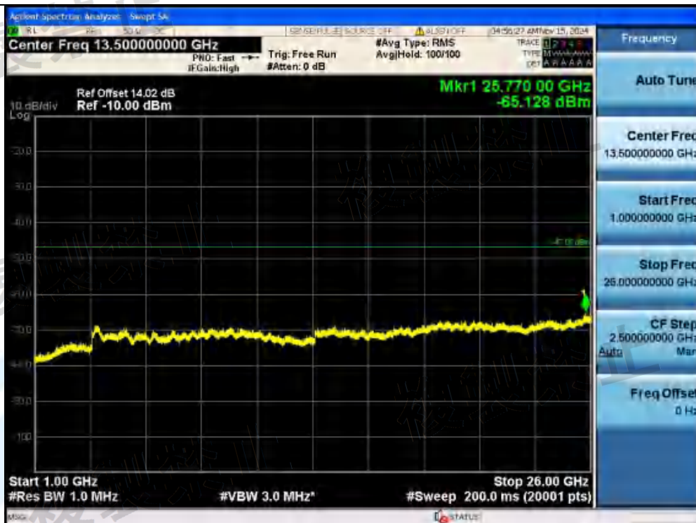
NTVN-11AX40MIMO-Ant1-5310-242Tone-RU62-1000~26000-PASS
