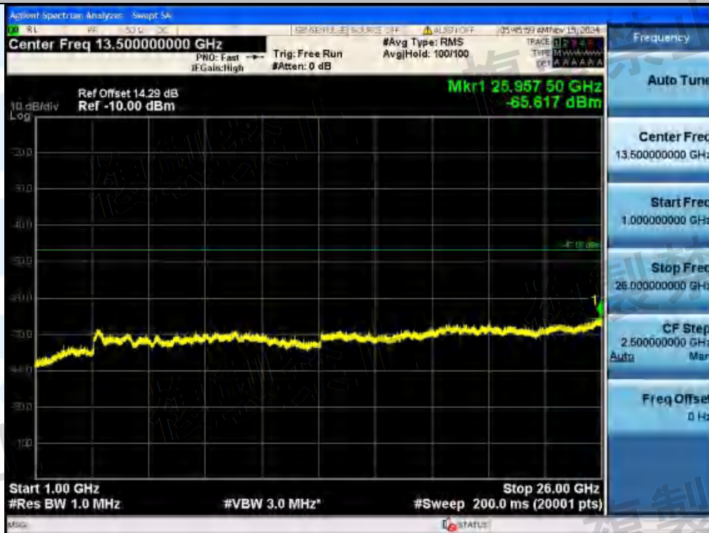
NTNV-11AX80MIMO-Ant2-5690-484Tone-RU65-1000~26000-PASS
