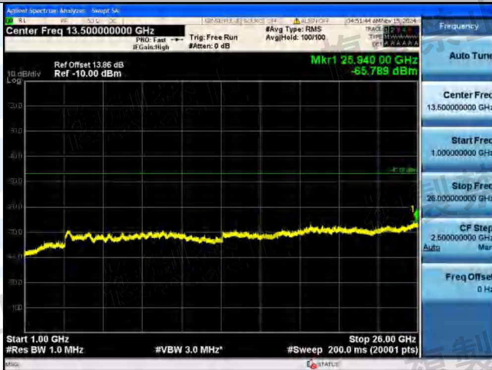
NTVN-11AX40MIMO-Ant2-5270-242Tone-RU61-1000~26000-PASS
