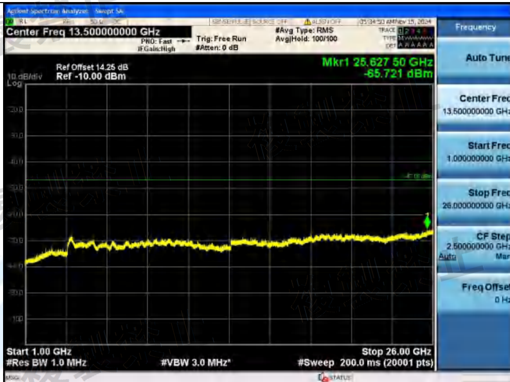
NTNV-11AX80MIMO-Ant1-5610-484Tone-RU66-1000~26000-PASS
