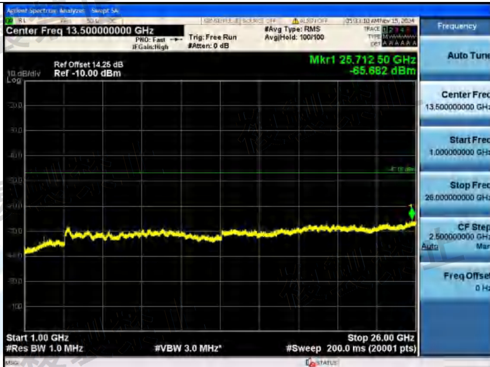
NTNV-11AX80MIMO-Ant1-5610-242Tone-RU64-1000~26000-PASS
