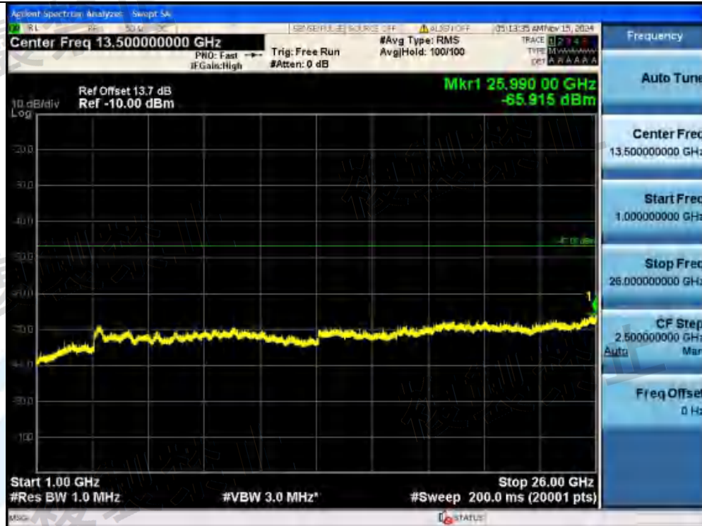
NTVN-11AX80MIMO-Ant1-5210-484Tone-RU65-1000~26000-PASS
