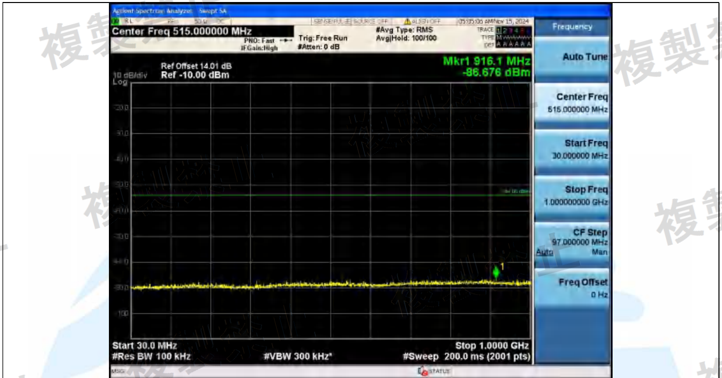
NTNV-11AX40MIMO-Ant1-5670-242Tone-RU61-30~1000-PASS
