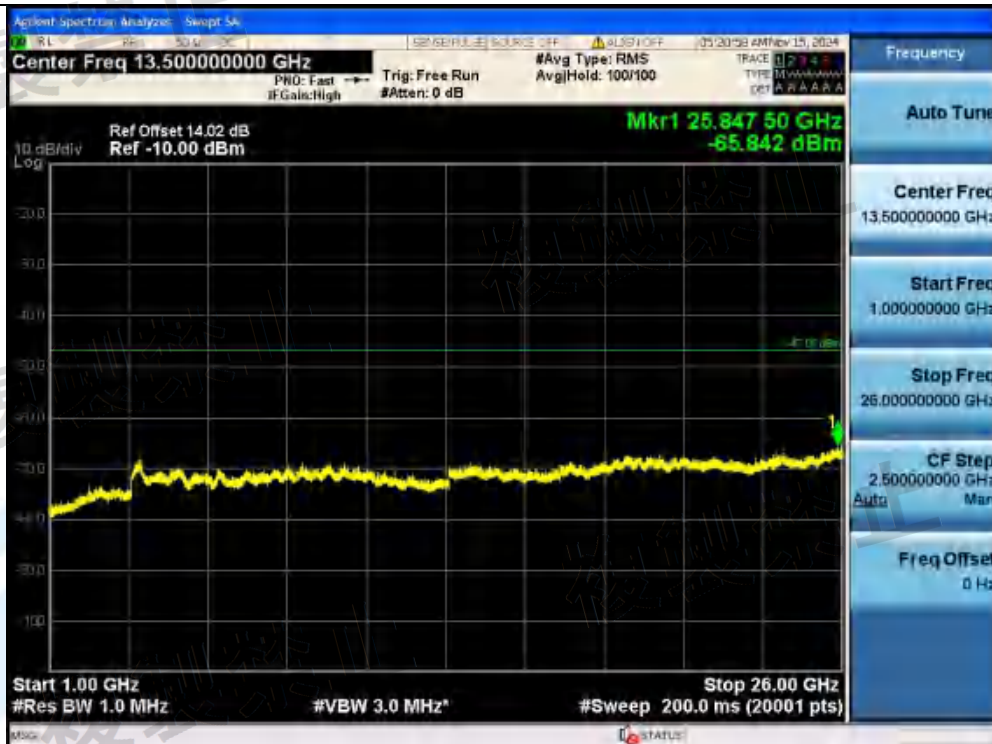
NTVN-11AX80MIMO-Ant1-5290-484Tone-RU66-1000~26000-PASS
