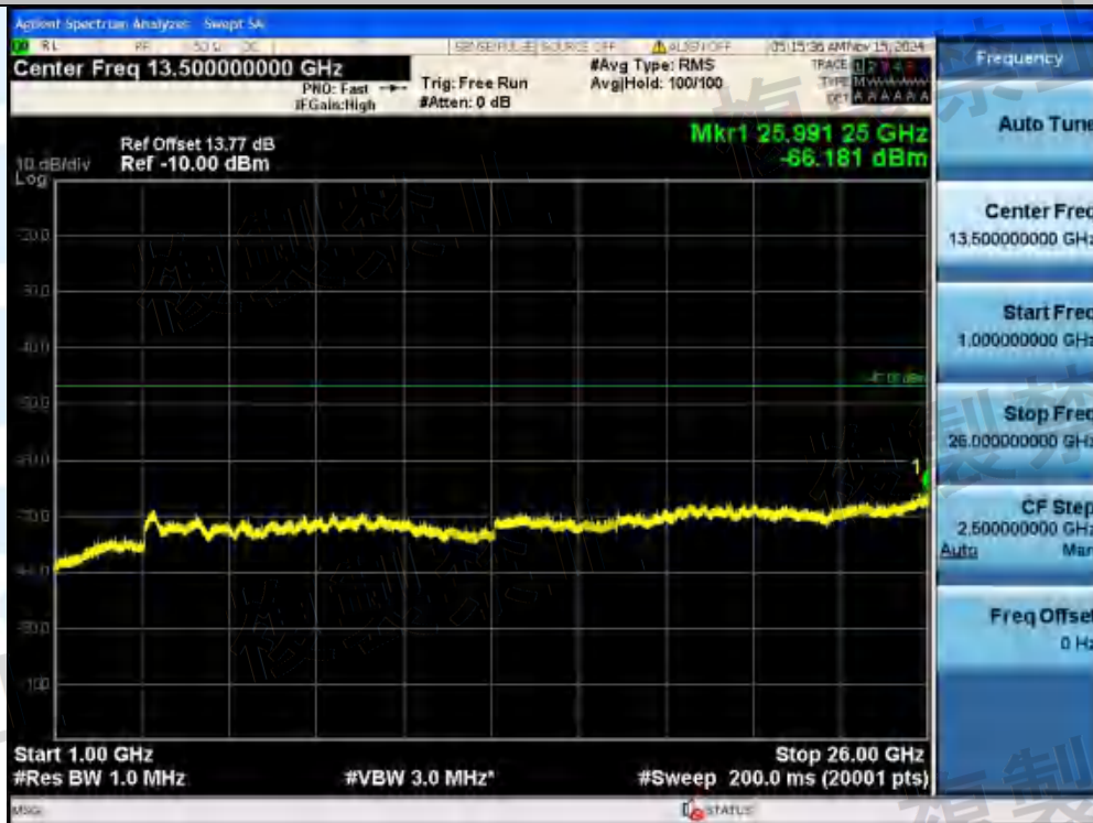
NTNV-11AX80MIMO-Ant2-5210-242Tone-RU61-1000~26000-PASS
