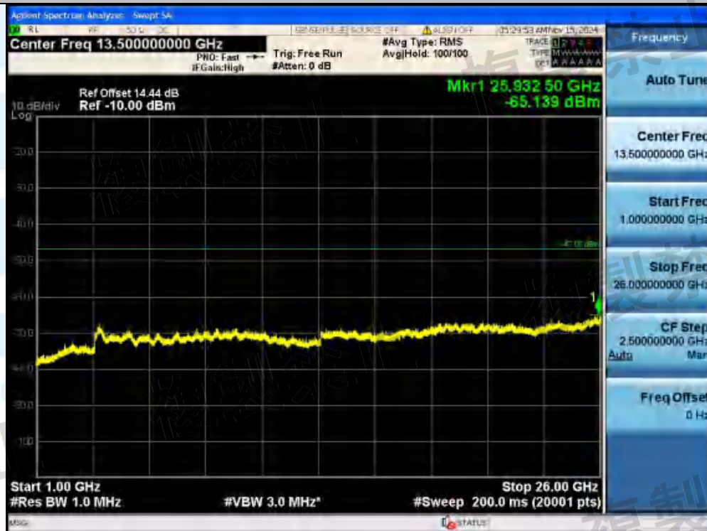
NTNV-11AX80MIMO-Ant2-5530-242Tone-RU61-1000~26000-PASS
