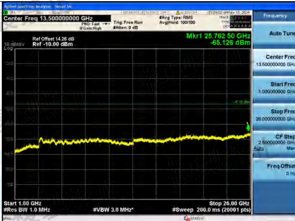
NTNV-11AX40MIMO-Ant1-5710-242Tone-RU62-1000~26000-PASS
