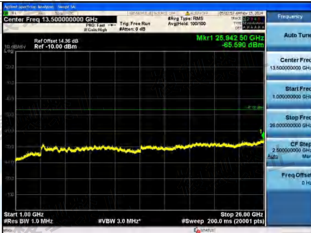
NTNV-11AX40MIMO-Ant1-5550-242Tone-RU62-1000~26000-PASS
