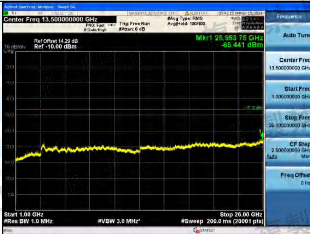
NTNV-11AX80MIMO-Ant2-5690-242Tone-RU61-1000~26000-PASS
