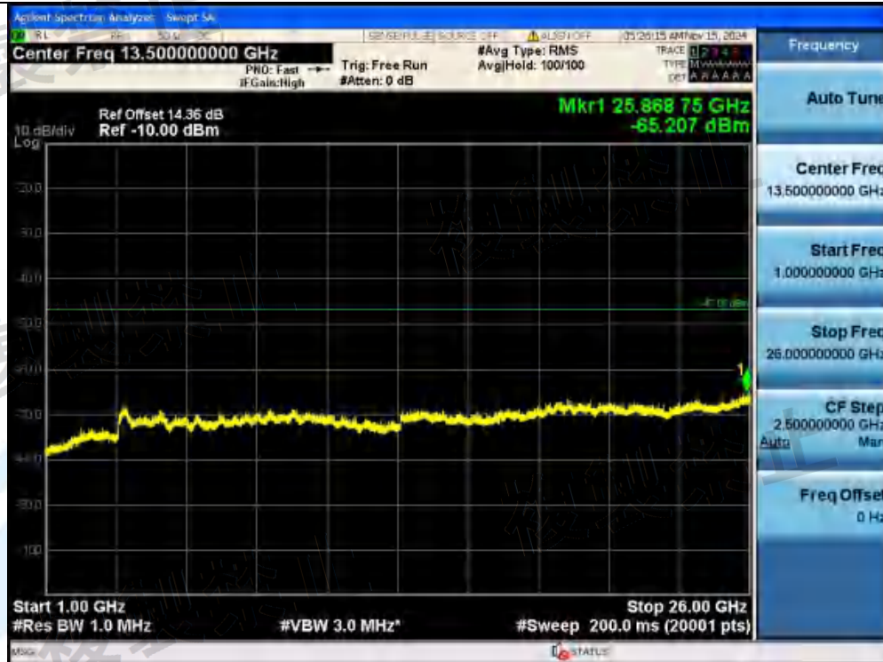
NTNV-11AX80MIMO-Ant1-5530-242Tone-RU61-1000~26000-PASS
