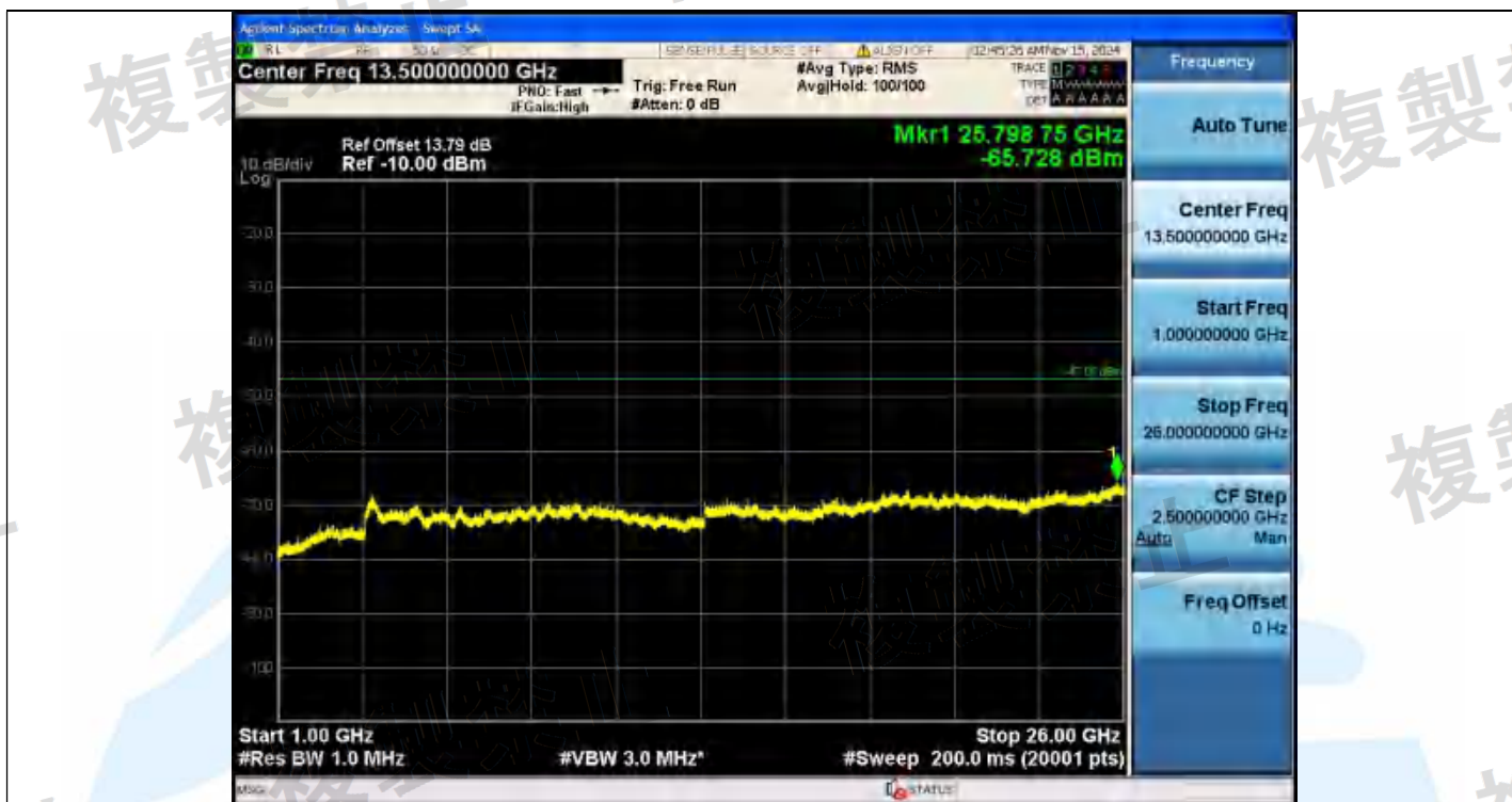
NTVN-11AX40MIMO-Ant1-5190-242Tone-RU61-1000~26000-PASS
