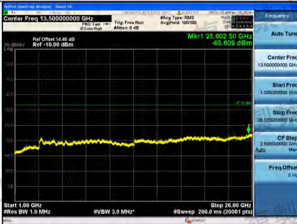
NTVN-11AX40MIMO-Ant2-5510-242Tone-RU61-1000~26000-PASS
