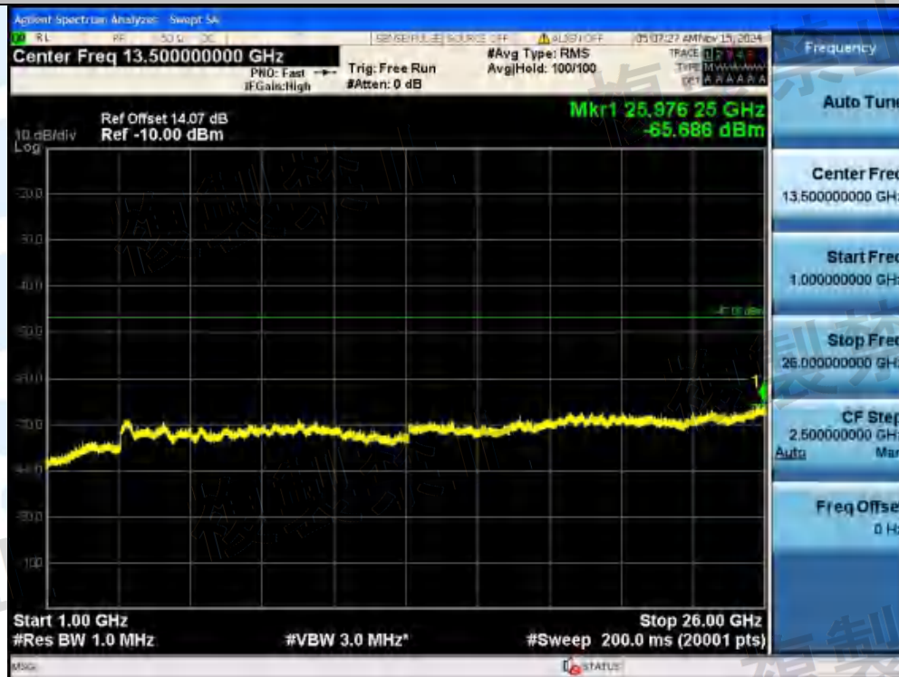
NTNV-11AX40MIMO-Ant2-5670-242Tone-RU61-1000~26000-PASS
