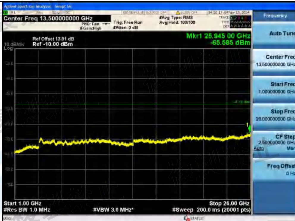
NTVN-11AX40MIMO-Ant1-5270-242Tone-RU61-1000~26000-PASS
