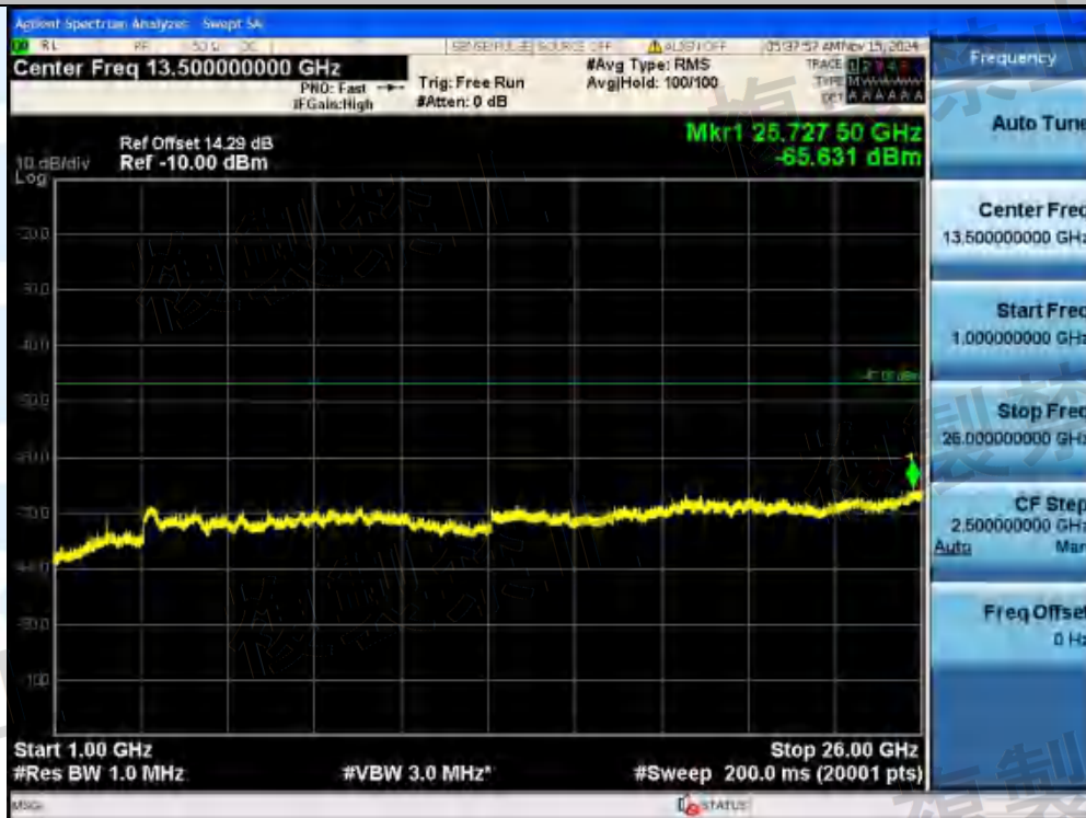
NTNV-11AX80MIMO-Ant2-5610-484Tone-RU66-1000~26000-PASS
