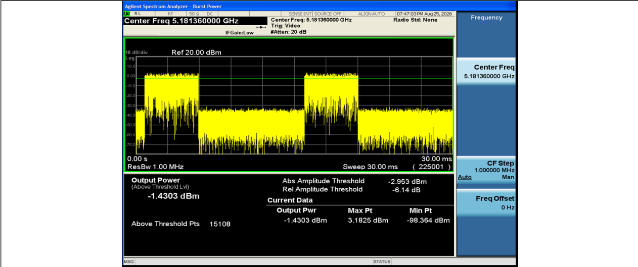
NTNV-11N20SISO-Ant1-5180-PASS
