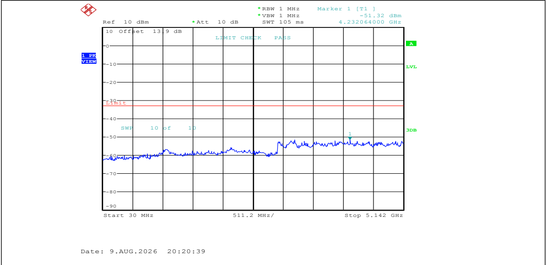
NTNV-11A-Ant1-5180-30~5142-PASS
