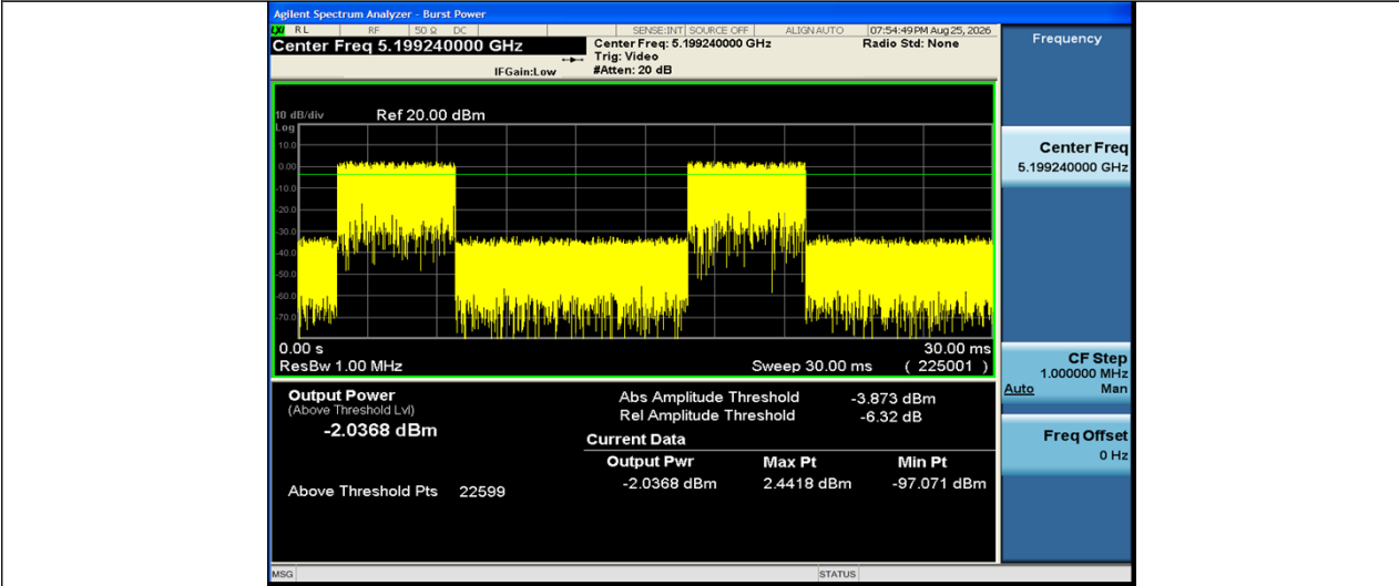
NTNV-11AC20SISO-Ant1-5200-PASS
