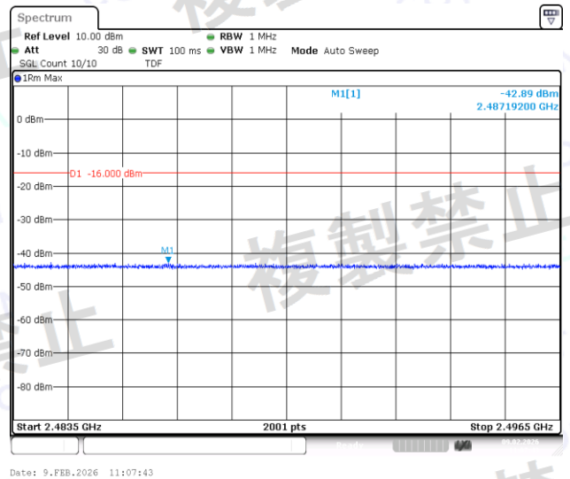
NTNV-BLE_2M-Ant1-2440-2483.5~2496.5-PASS
