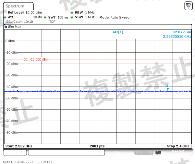
NTVN-BLE_2M-Ant1-2404-2387~2400-PASS
