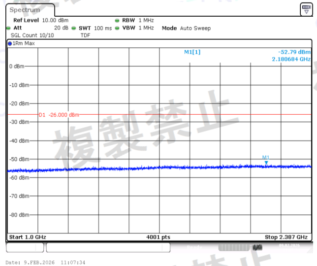
NTNV-BLE_2M-Ant1-2440-1000~2387-PASS
