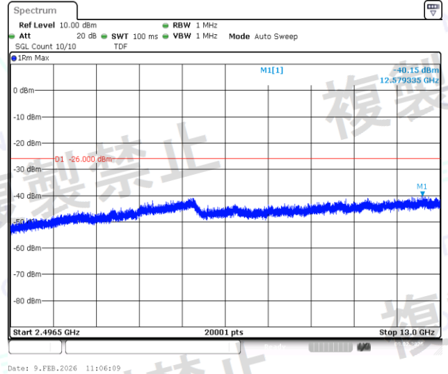
NTNV-BLE_2M-Ant1-2404-2496.5~13000-PASS
