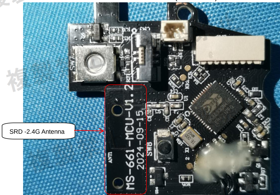
INTERNAL VIEW OF EUT (FIGURE 13)
