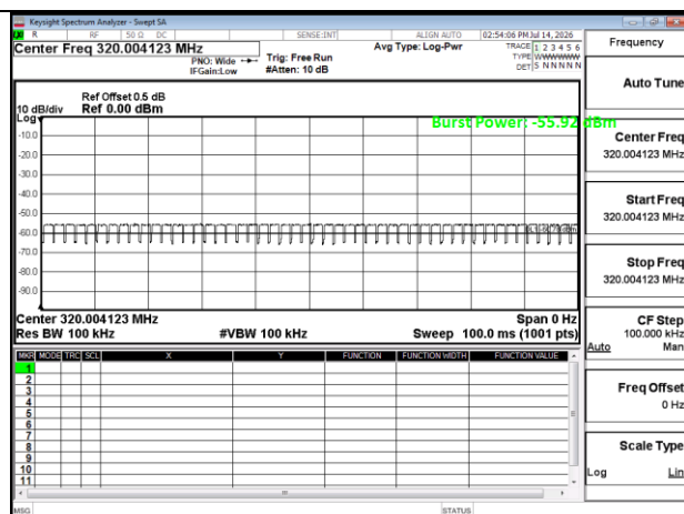
RX Below 1GHz BLE 1M 2402MHz Sample
