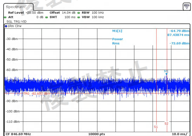
NTNV-11AC20MIMO-Ant1-5260-30~1000-PASS
