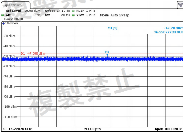
NTNV-11AC20MIMO-Ant2-5300-1000~26000-PASS
