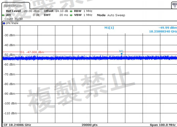
NTNV-11AC20MIMO-Ant2-5260-1000~26000-PASS
