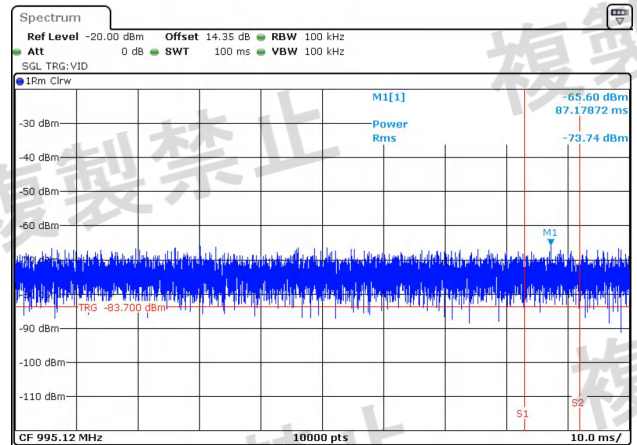
NTNV-11AC20MIMO-Ant2-5320-30~1000-PASS
