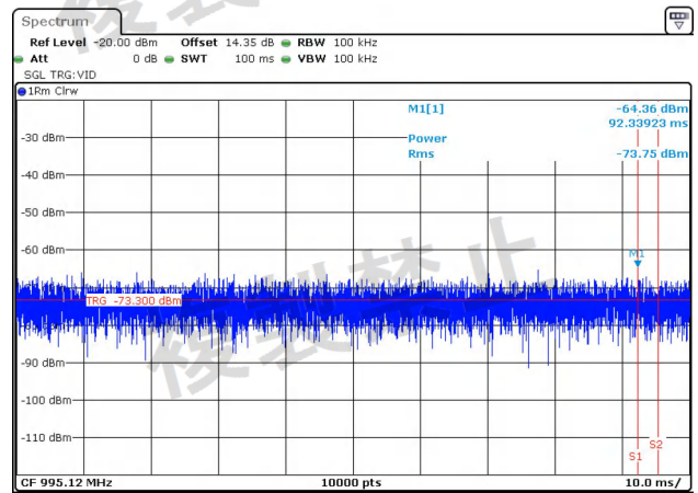
NTNV-11AC20MIMO-Ant2-5320-30~1000-PASS
