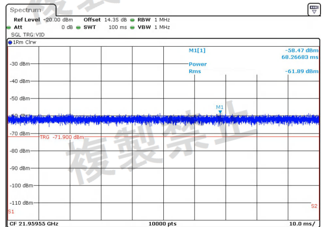
NTNV-11AC20MIMO-Ant2-5320-1000~26000-PASS
