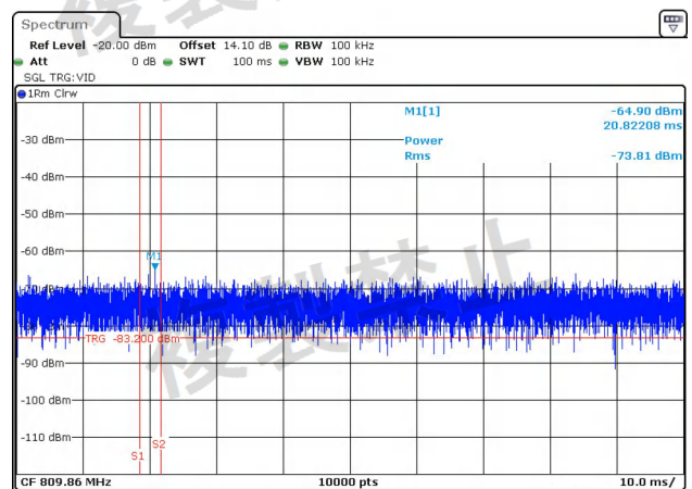
NTNV-11N40MIMO-Ant2-5310-30~1000-PASS
