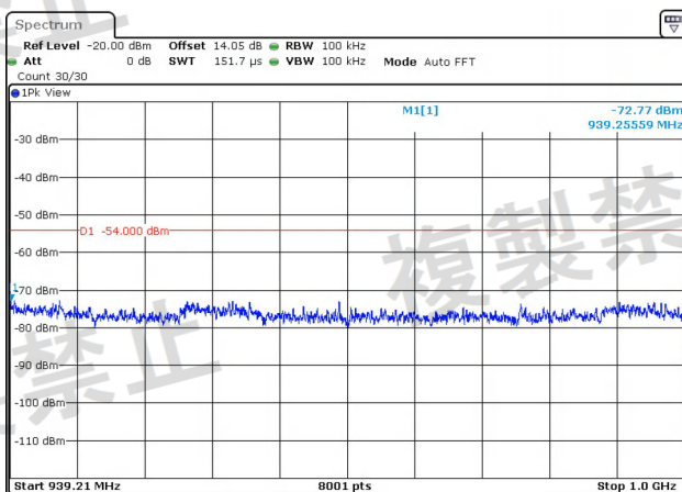
NTNV-11N40MIMO-Ant2-5310-30~1000-PASS
