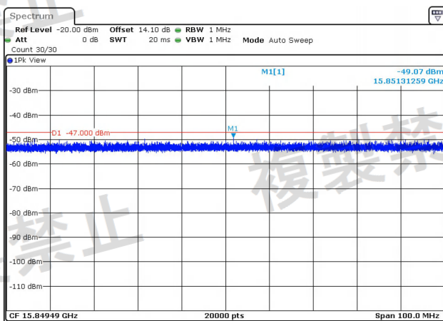
NTNV-11N40MIMO-Ant1-5270-1000~26000-PASS
