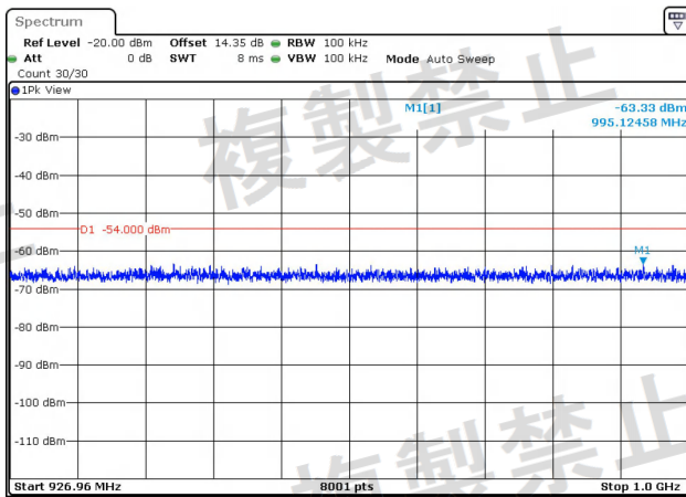
NTNV-11AC20MIMO-Ant2-5320-30~1000-PASS
