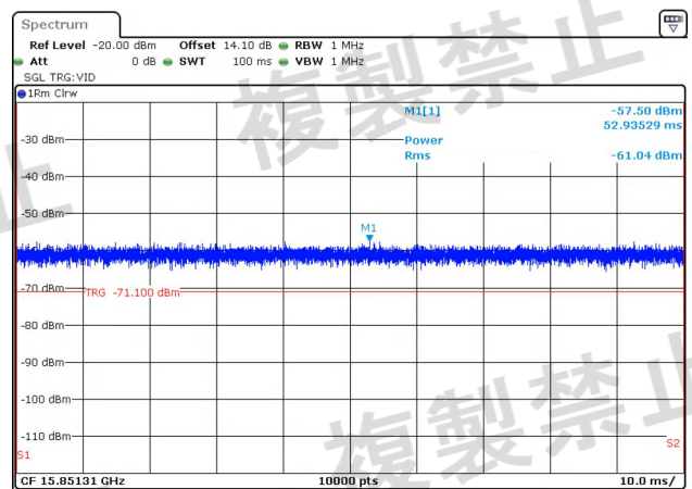
NTNV-11N40MIMO-Ant1-5270-1000~26000-PASS
