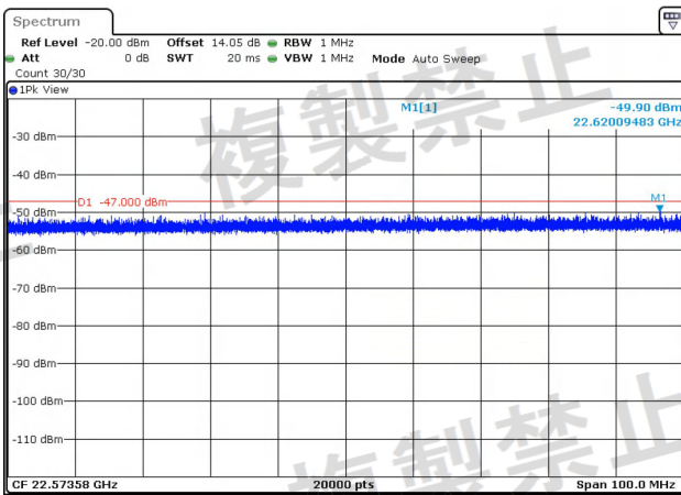
NTNV-11AC20MIMO-Ant1-5300-1000~26000-PASS
