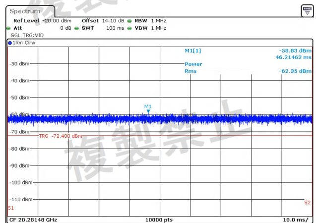
NTNV-11N40MIMO-Ant2-5310-1000~26000-PASS
