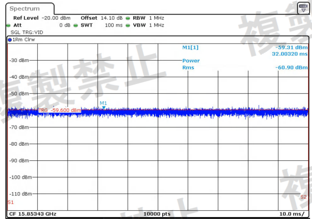
NTNV-11N40-Ant2-5310-1000~26000-PASS
