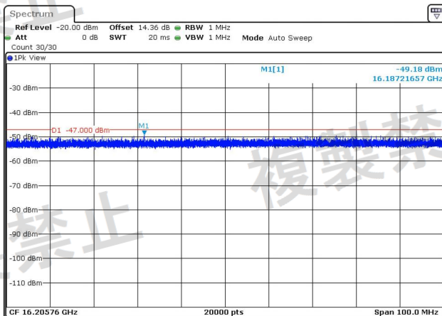
NTNV-11AC20MIMO-Ant2-5320-1000~26000-PASS
