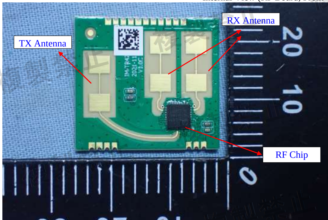
Figure 9 Internal View (RF Board, Front View)
