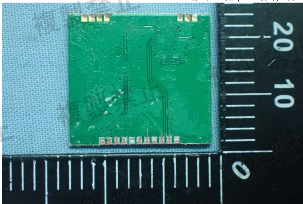
Figure 8 Internal View (RF Board, Back View)
