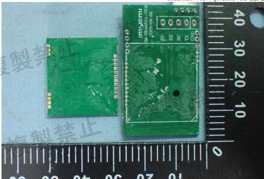
Figure 7 Internal View (Removed RF Board)
