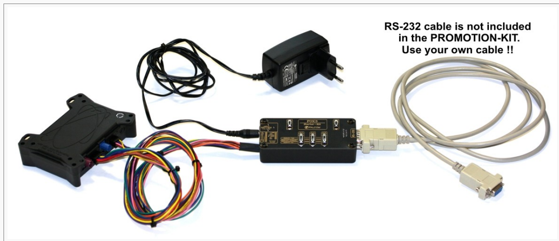
Figure 5: Overview of PROMOTION-KIT setup
