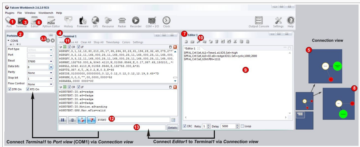
Figure 8: FALCOM Workbench software.
