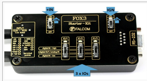
Figure 10: Top panel of the control-box.
