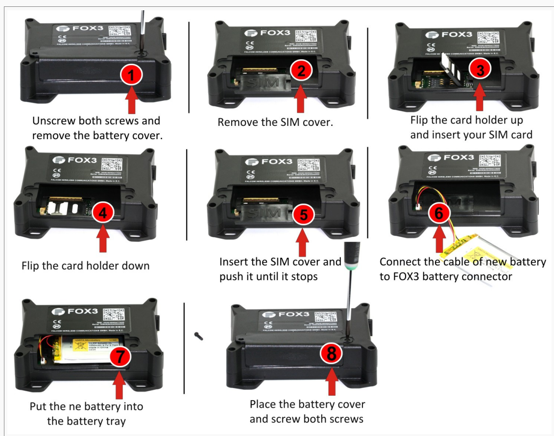
Figure 13: Inserting your SIM card and replacing the battery by a new one
