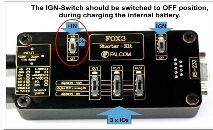
Figure 6: Overview of the control-box top panel (+IN = ON)
