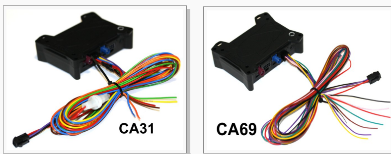
Figure 12: Supplied cables (a reference to the colours and pinout is provided in Table 7 and Table 8 )
