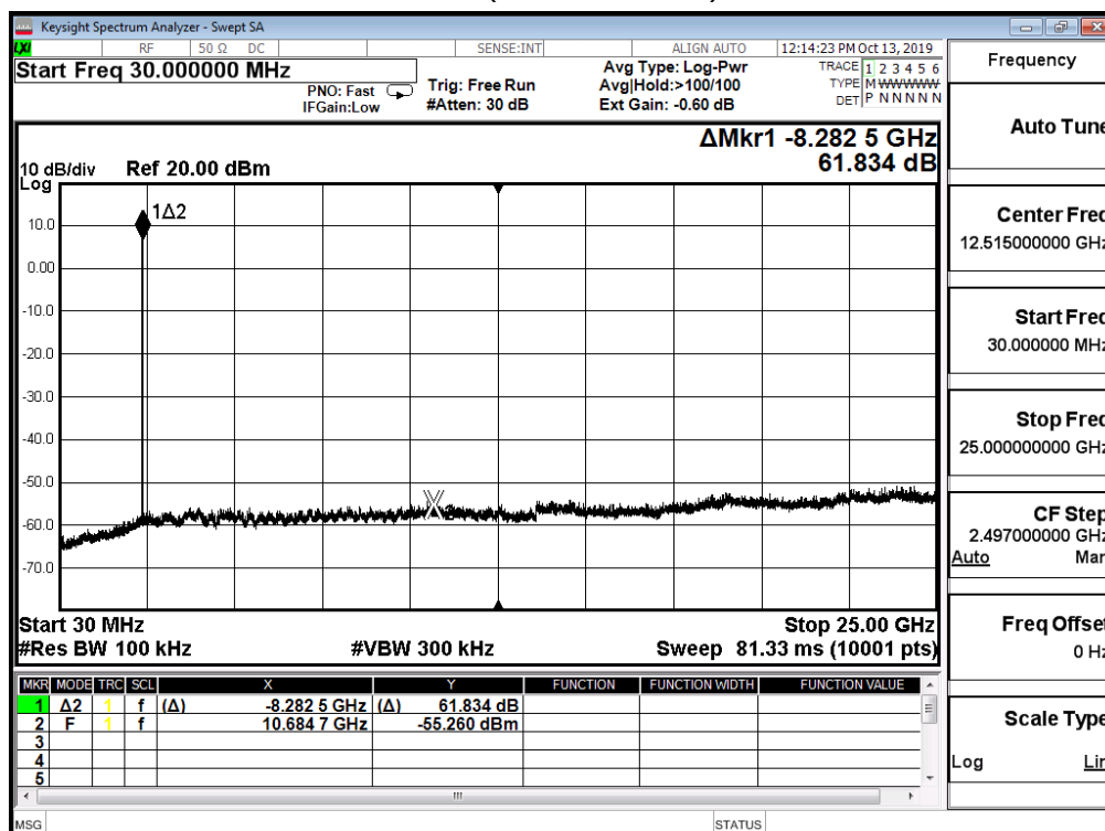
Channel 39 (30MHz-25GHz)-GFSK
