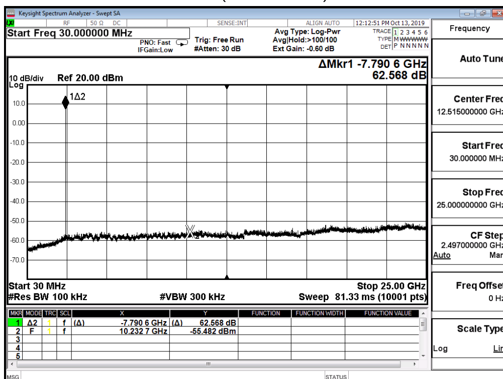
Channel 39 (30MHz-25GHz)-GFSK
