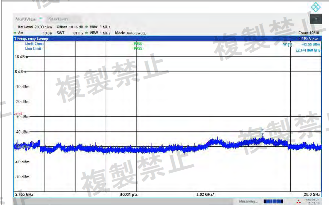
NTNV-11N20MIMO-Ant1-5580-5765~26000-PASS
