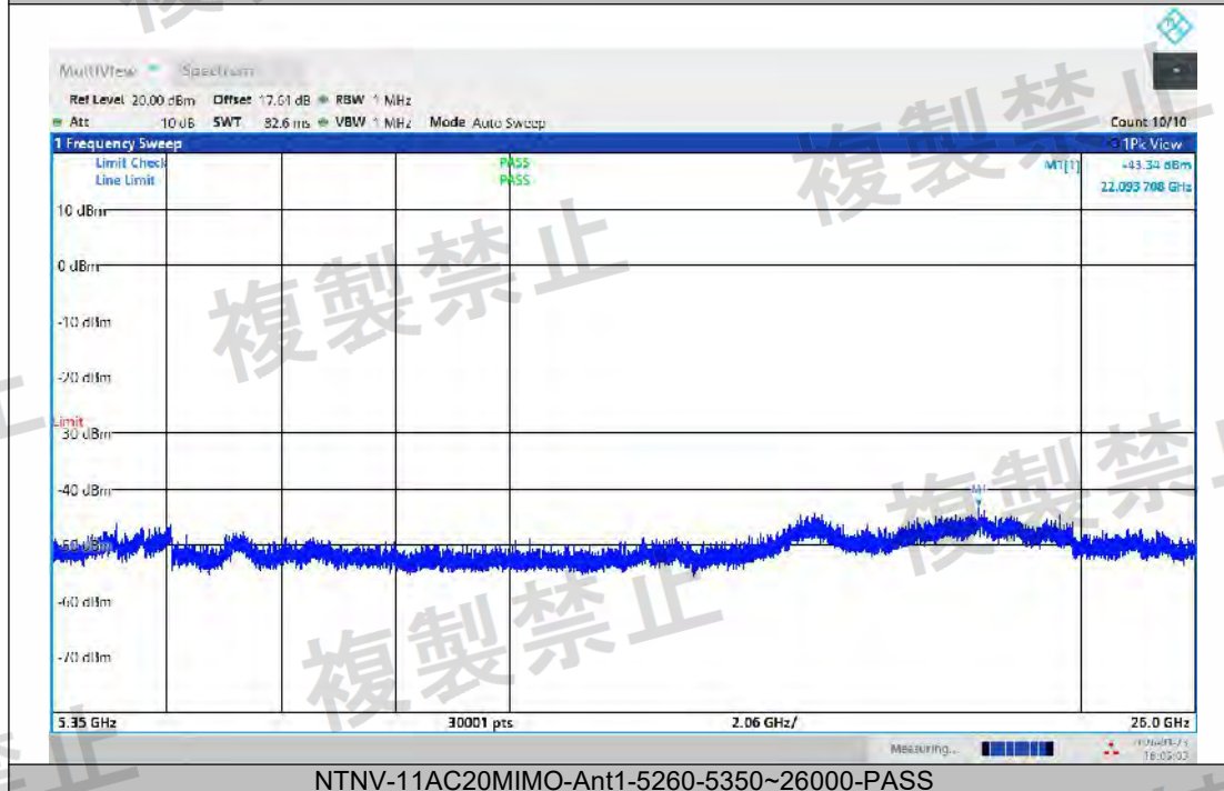
NTNV-11AC20MIMO-Ant1-5260-5350~26000-PASS
