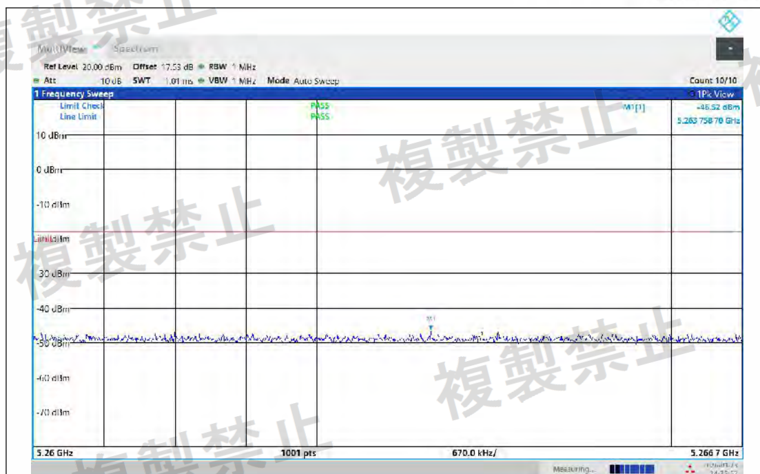
NTNV-11N20MIMO-Ant2-5180-5260~5266.7-PASS
