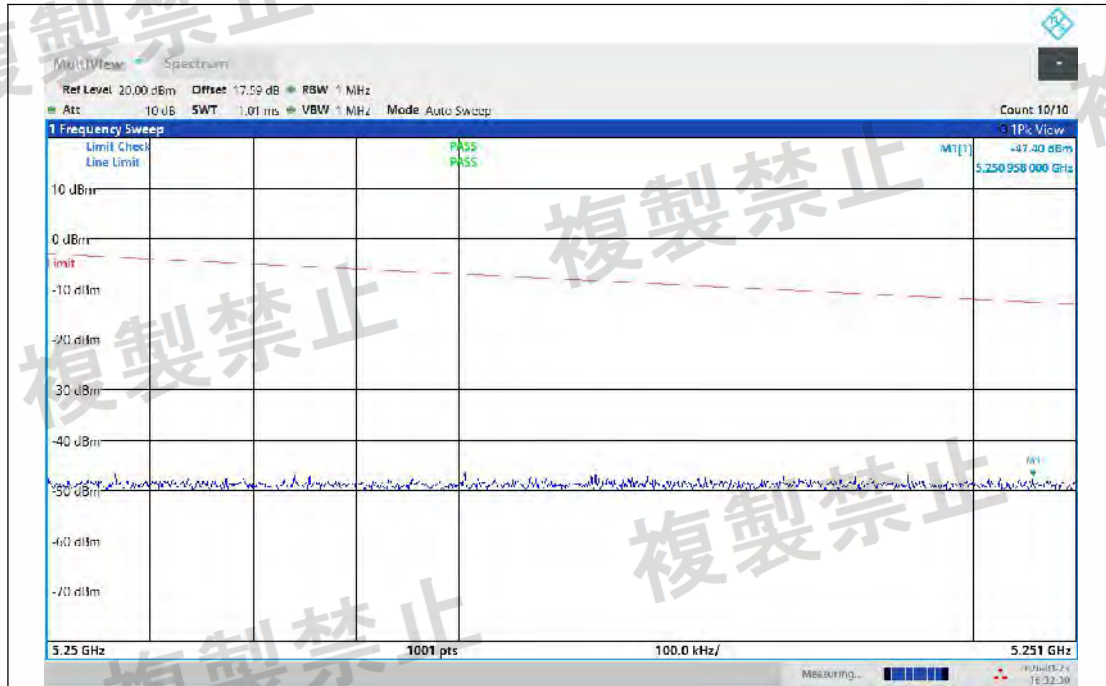
NTNV-11AC40MIMO-Ant2-5190-5250~5251-PASS
