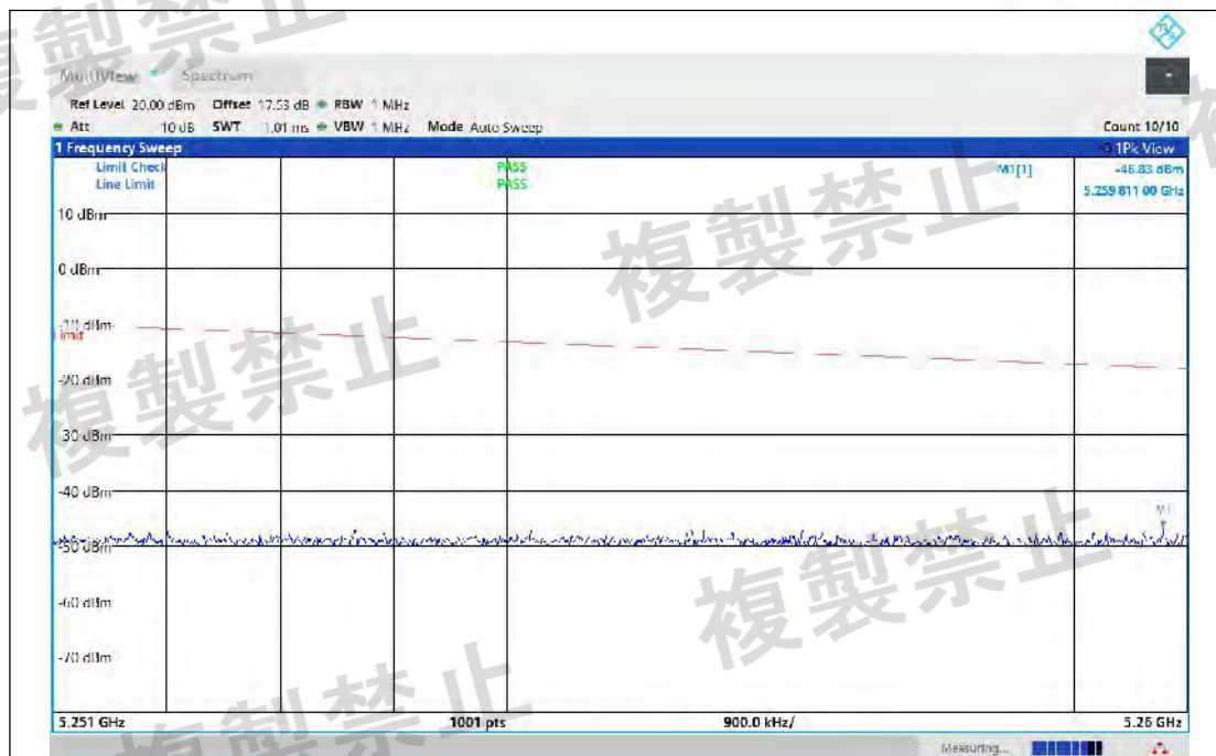
NTNV-11AX20MIMO-Ant2-5180-5251~5260-PASS
