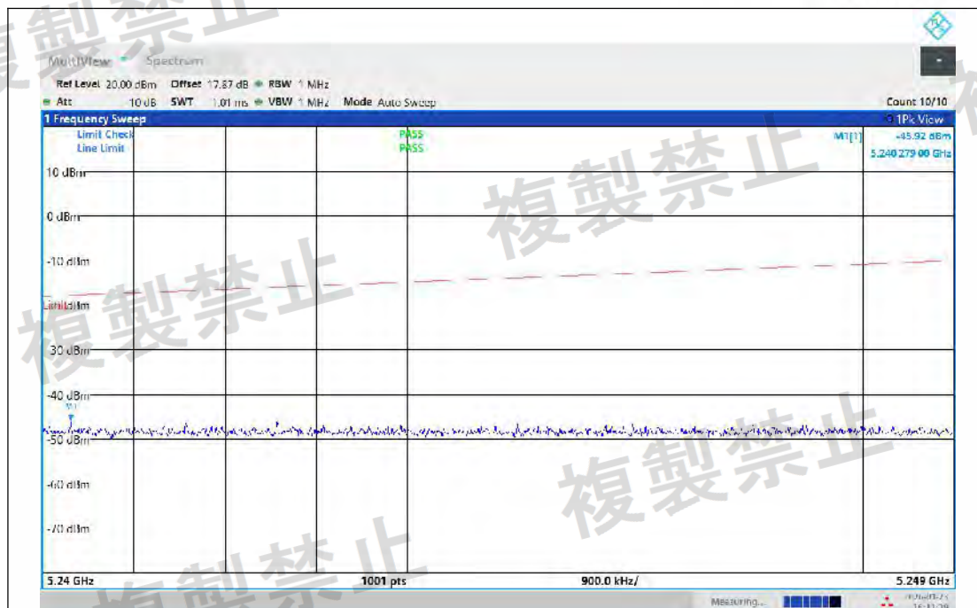
NTNV-11AC20MIMO-Ant2-5280-5240~5249-PASS
