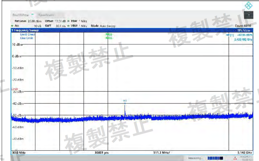
NTNV-11AC20MIMO-Ant1-5180-30~5142-PASS
