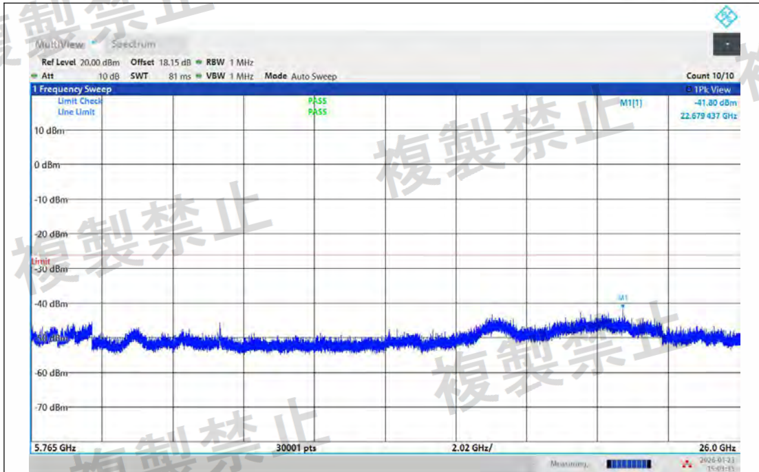
NTNV-11N20MIMO-Ant2-5580-5765~26000-PASS
