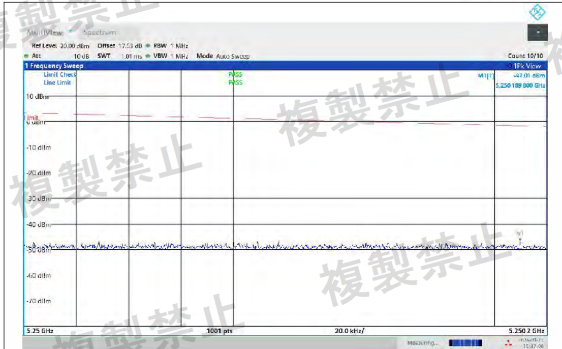
NTNV-11AC20MIMO-Ant2-5180-5250~5250.2-PASS
