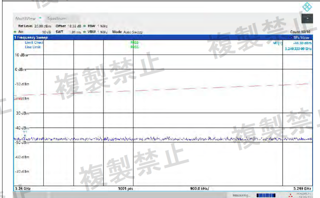
NTNV-11AC20MIMO-Ant1-5320-5240~5249-PASS
