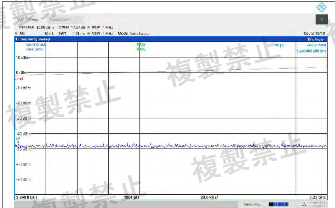
NTNV-11N20MIMO-Ant2-5280-5249.8~5250-PASS
