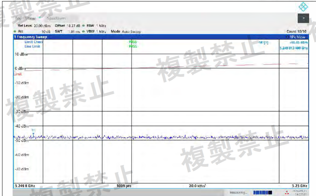
NTNV-11N20MIMO-Ant2-5320-5249.8~5250-PASS
