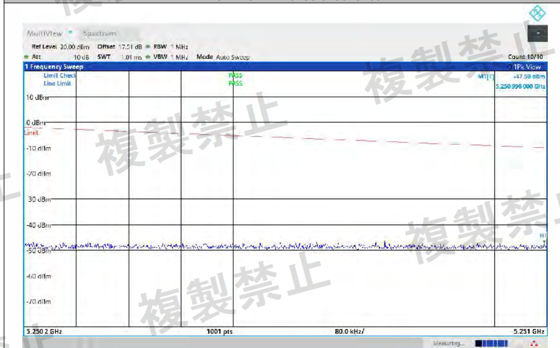
NTNV-11AX20MIMO-Ant1-5180-5250.2~5251-PASS
