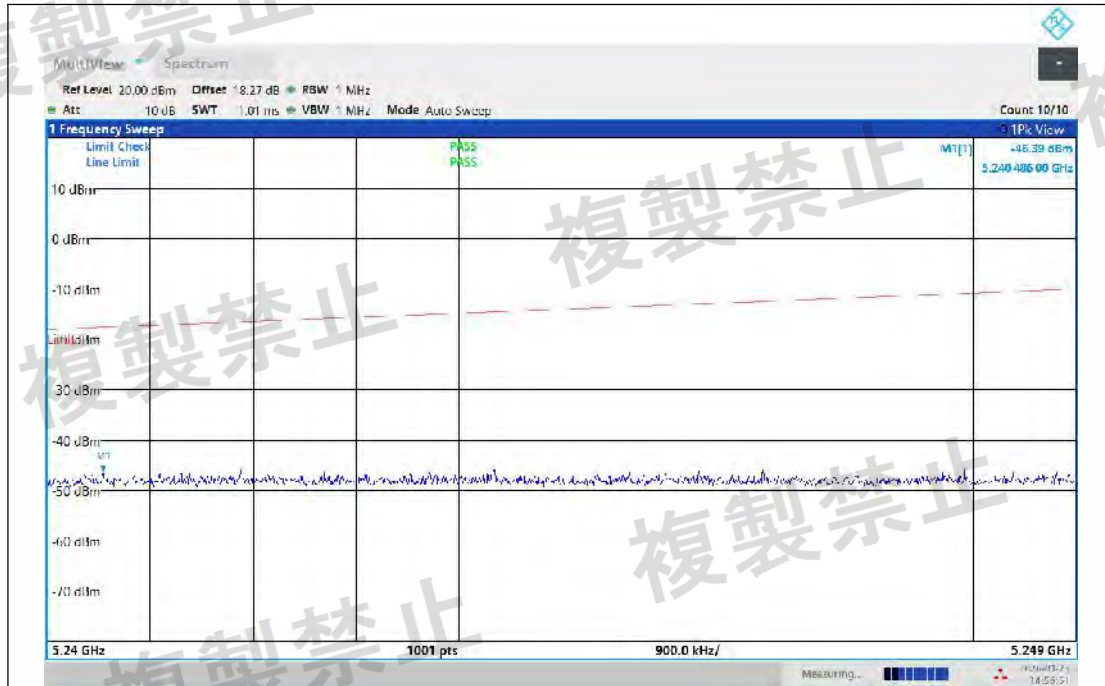
NTNV-11N20MIMO-Ant2-5320-5240~5249-PASS
