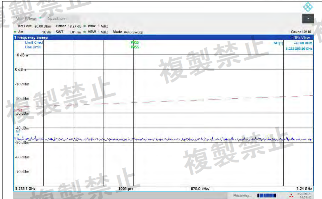
NTNV-11N20MIMO-Ant2-5320-5233.3~5240-PASS
