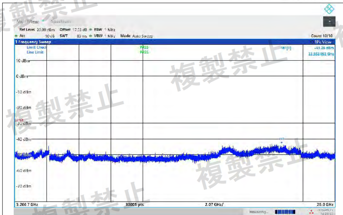
NTNV-11N20MIMO-Ant2-5180-5266.7~26000-PASS
