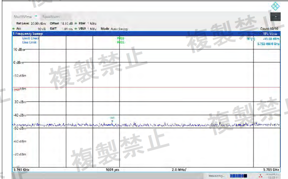
NTNV-11N20MIMO-Ant1-5580-5745~5765-PASS
