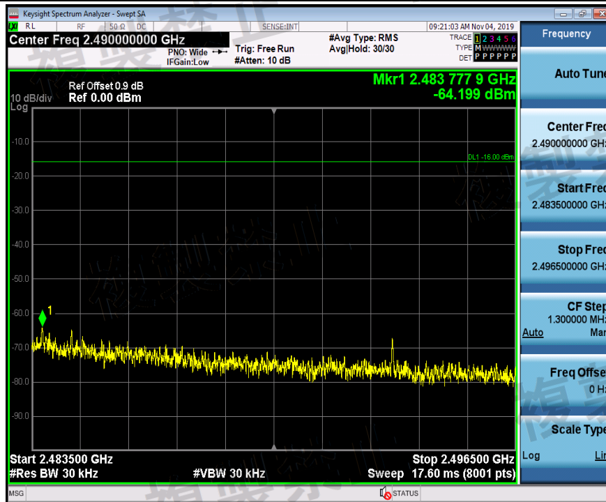
TNVL_DH5_Ant1_2480_2483.5~2496.5
