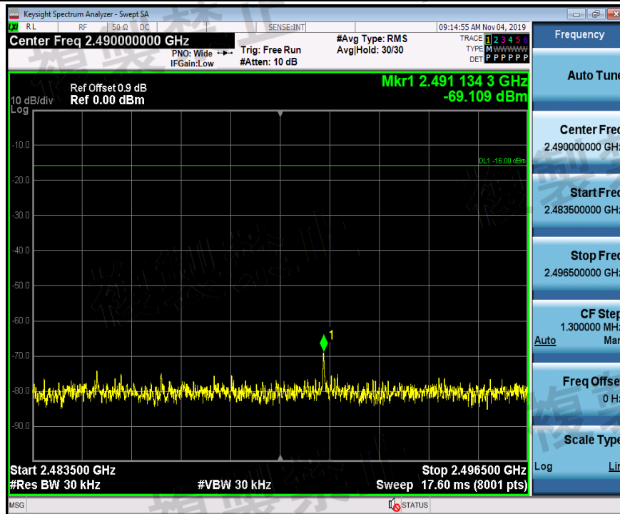
TNVL_2DH5_Ant1_2441_2483.5~2496.5
