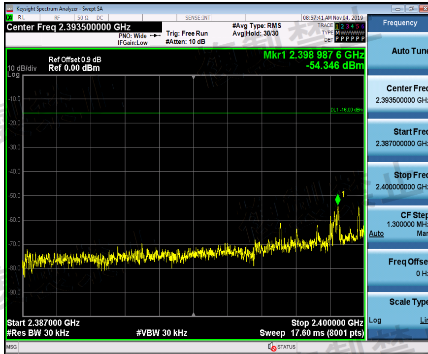
TNVL_2DH5_Ant1_2402_2387~2400
