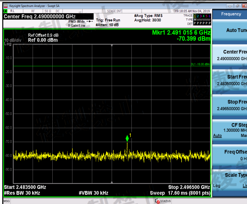
TNVL_3DH5_Ant1_2441_2483.5~2496.5
