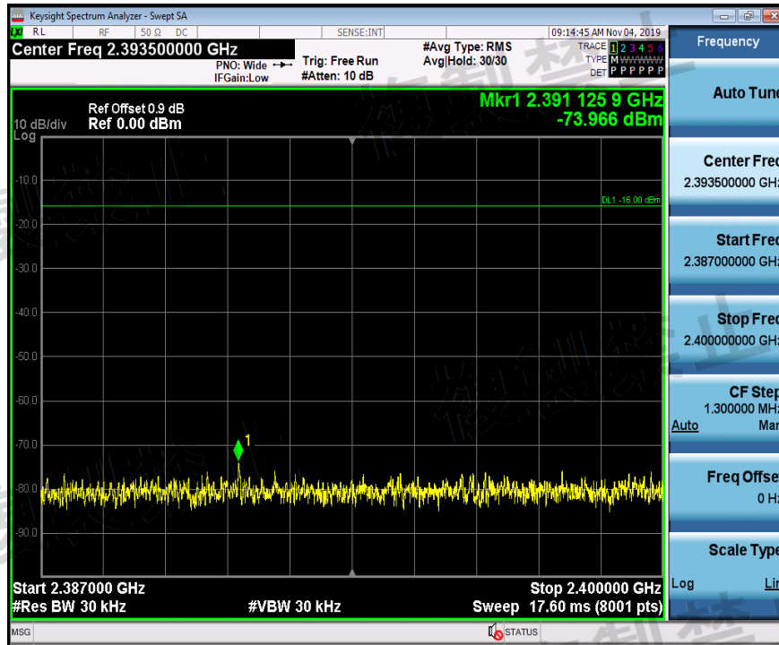
TNVL_2DH5_Ant1_2441_2387~2400
