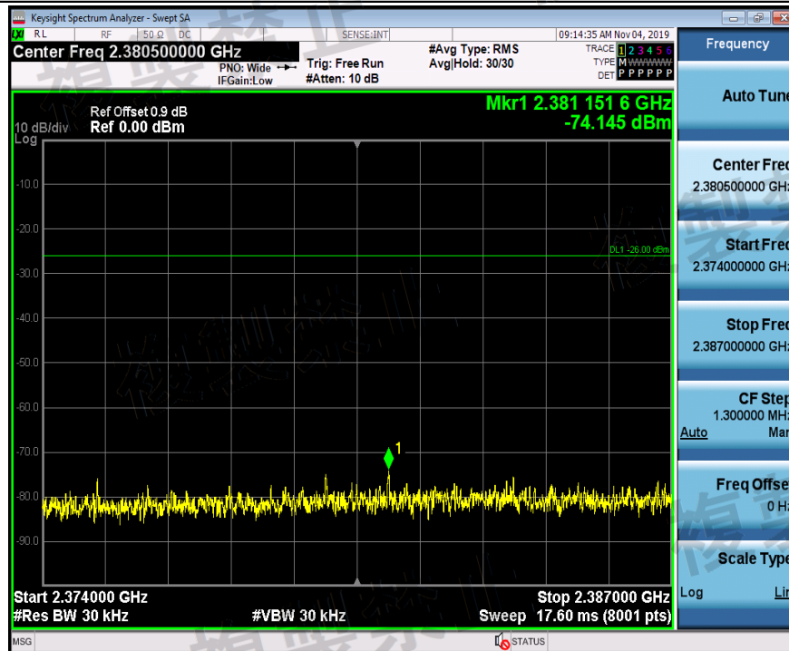
TNVL_2DH5_Ant1_2441_2374~2387
