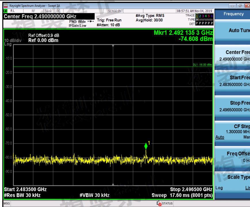
TNVL_2DH5_Ant1_2402_2483.5~2496.5
