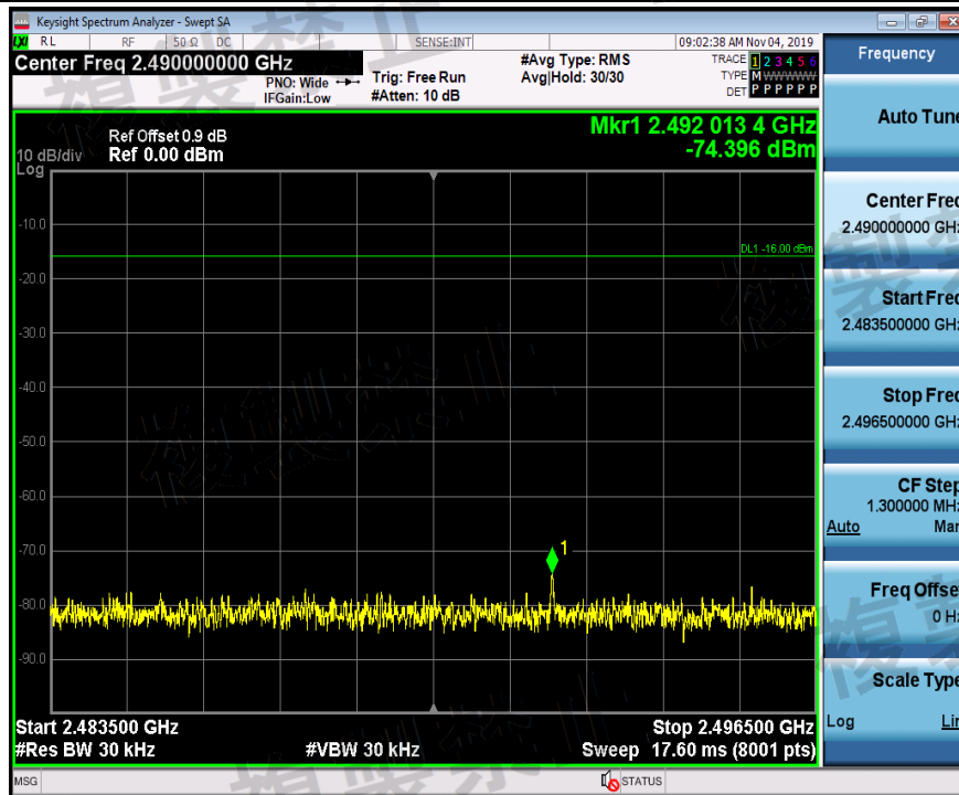
TNVL_3DH5_Ant1_2402_2483.5~2496.5
