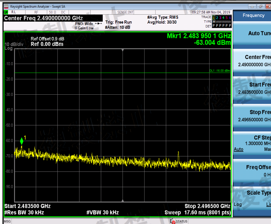
TNVL_3DH5_Ant1_2480_2483.5~2496.5
