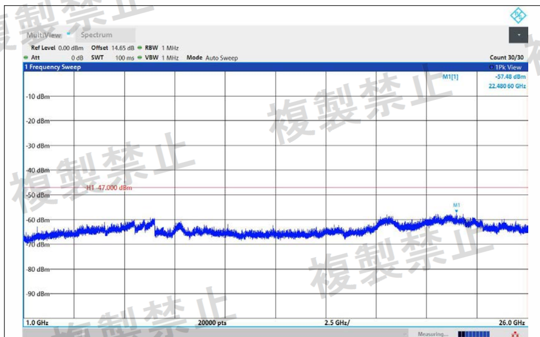
NTNV-11AC40MIMO-Ant1-5510-1000~26000-PASS
