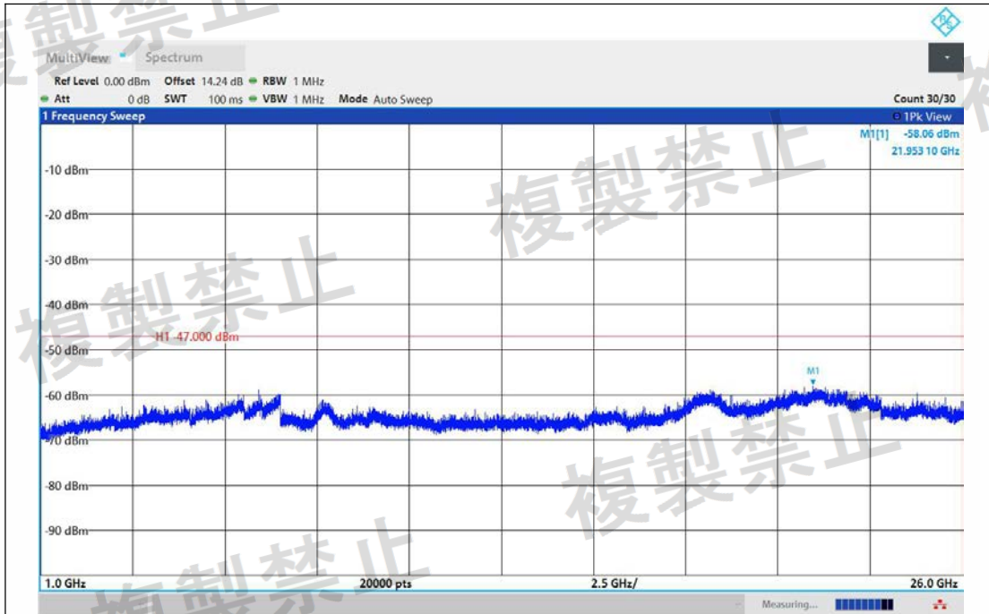
NTNV-11AC160MIMO-Ant1-5570-1000~26000-PASS
