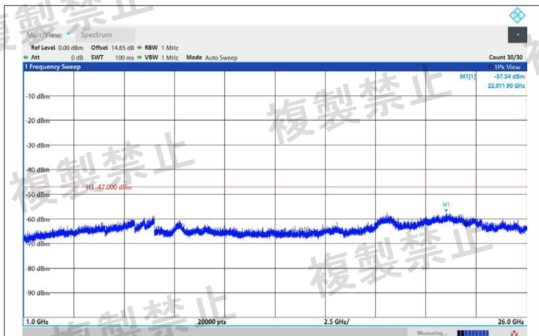
NTNV-11AX40MIMO-Ant1-5510-1000~26000-PASS
