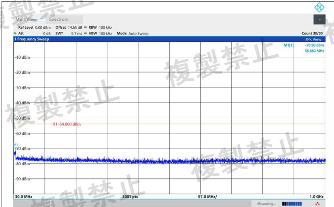
NTNV-11AX40MIMO-Ant1-5510-30~1000-PASS
