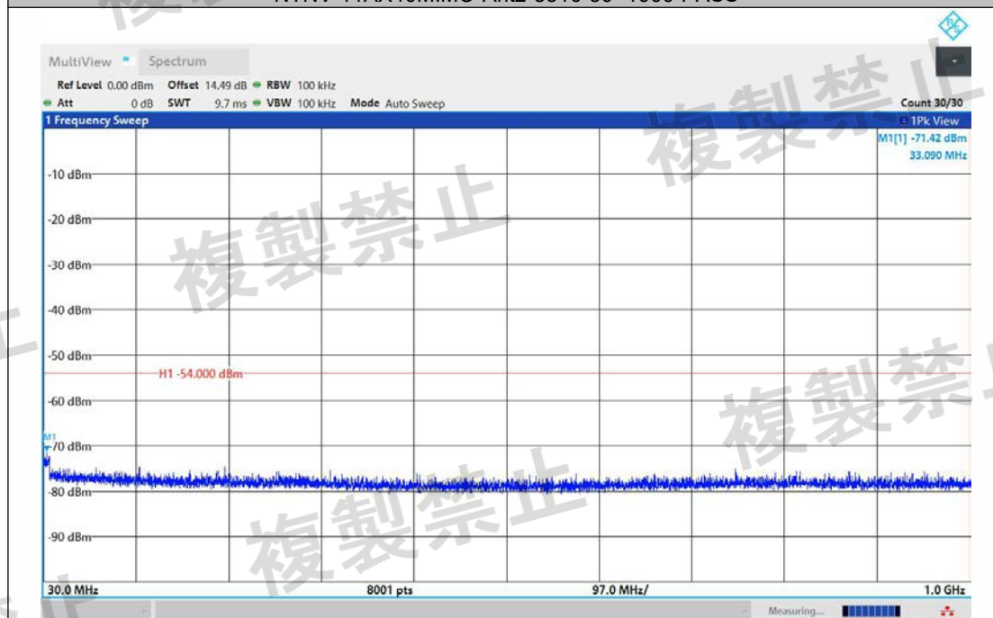
NTNV-11AX40MIMO-Ant1-5310-30~1000-PASS
