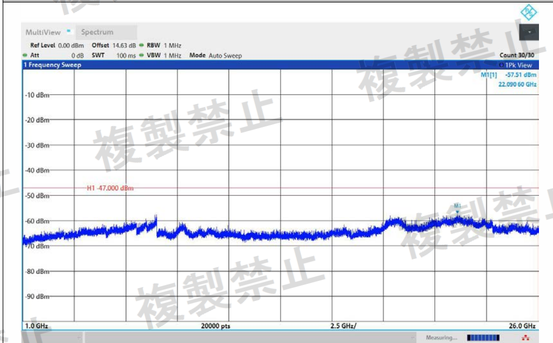
NTNV-11AC80MIMO-Ant2-5530-1000~26000-PASS
