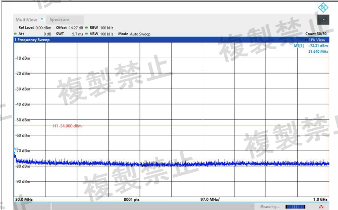
NTNV-11AX20MIMO-Ant2-5260-30~1000-PASS
