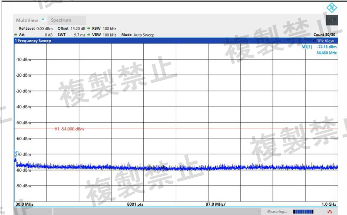
NTNV-11AX80MIMO-Ant2-5610-30~1000-PASS
