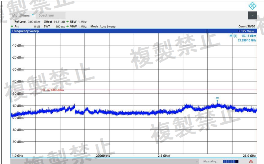
NTNV-11AC20MIMO-Ant1-5700-1000~26000-PASS
