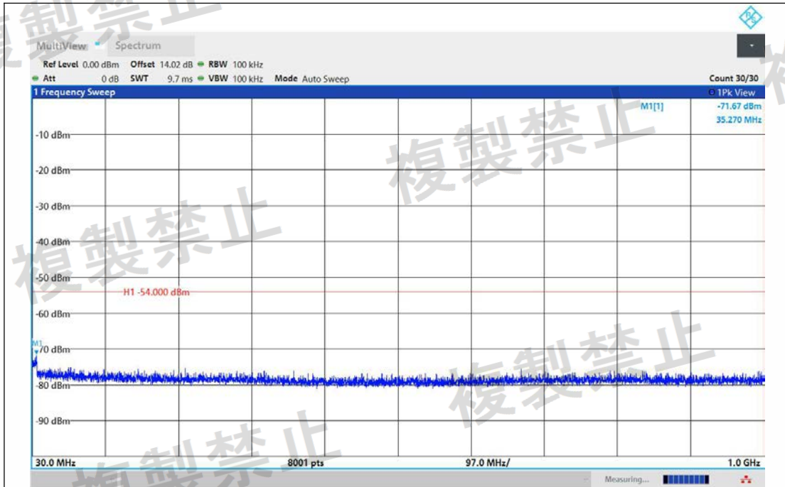
NTNV-11AX160MIMO-Ant1-5250-30~1000-PASS
