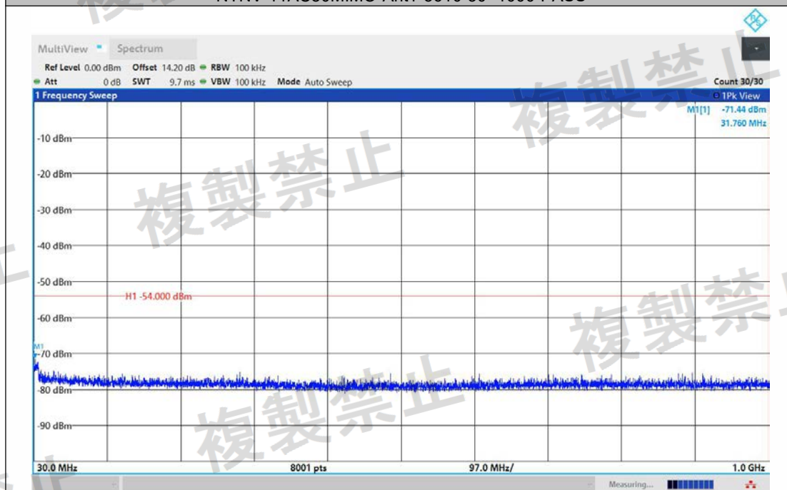
NTNV-11AC80MIMO-Ant2-5610-30~1000-PASS
