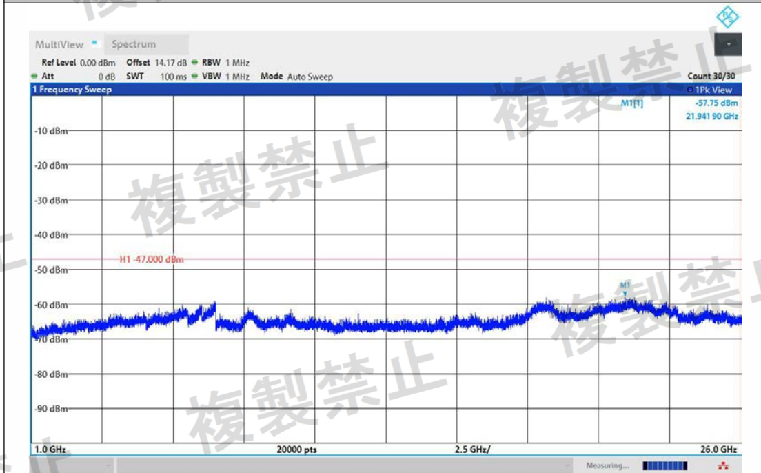
NTNV-11AC80MIMO-Ant2-5290-1000~26000-PASS
