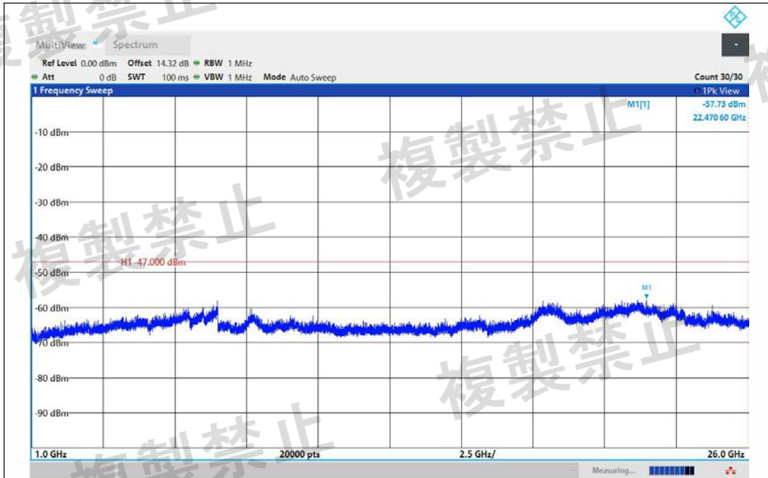
NTNV-11AC40MIMO-Ant1-5270-1000~26000-PASS
