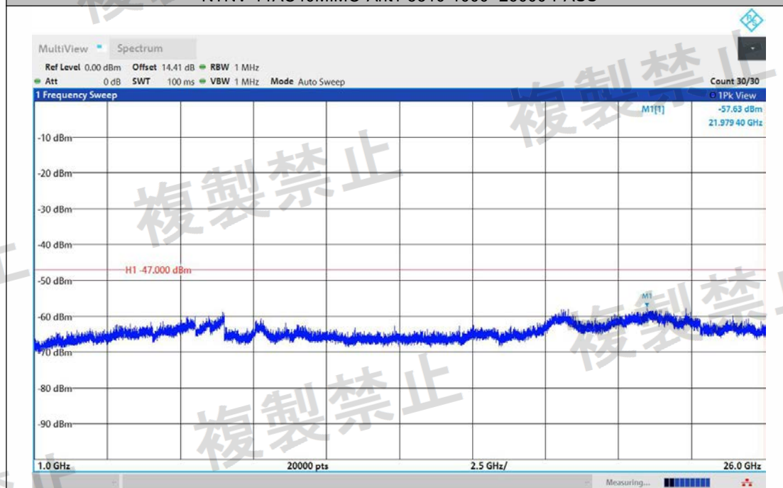
NTNV-11AC40MIMO-Ant2-5310-1000~26000-PASS
