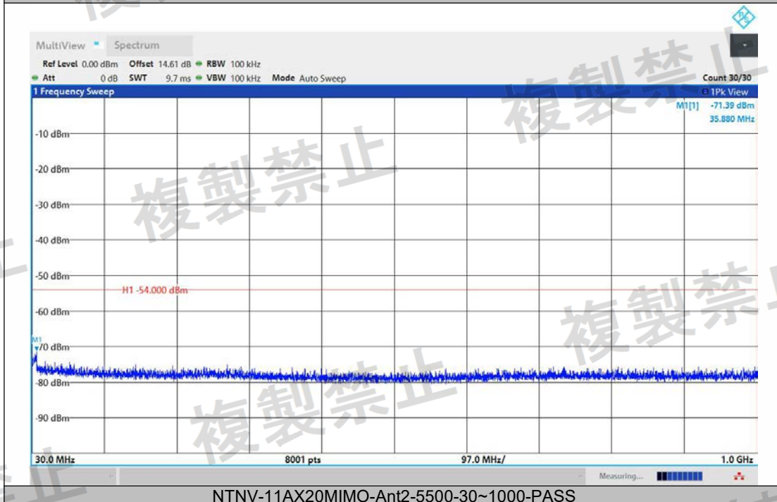
NTN-11AX20MIMO-Ant2-5500-30~1000-PASS
