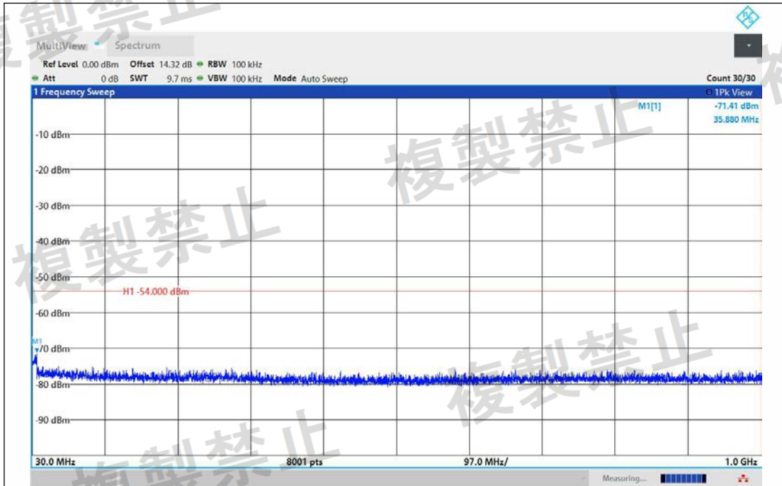
NTVN-11AC40MIMO-Ant1-5270-30~1000-PASS
