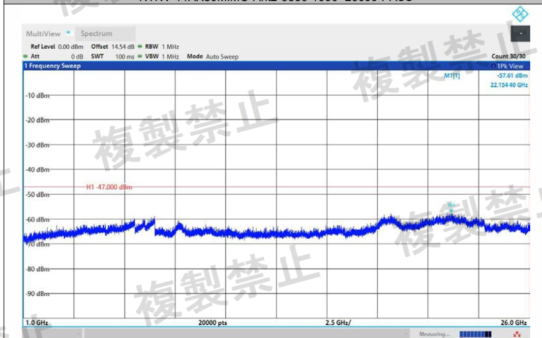
NTNV-11AX80MIMO-Ant1-5530-1000~26000-PASS
