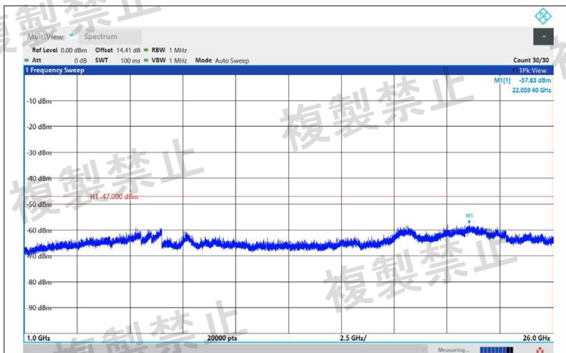
NTNV-11AX20MIMO-Ant1-5700-1000~26000-PASS
