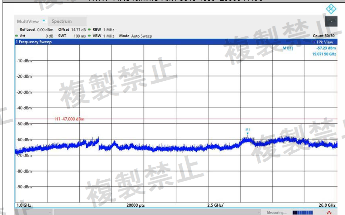
NTNV-11AC40MIMO-Ant2-5510-1000~26000-PASS
