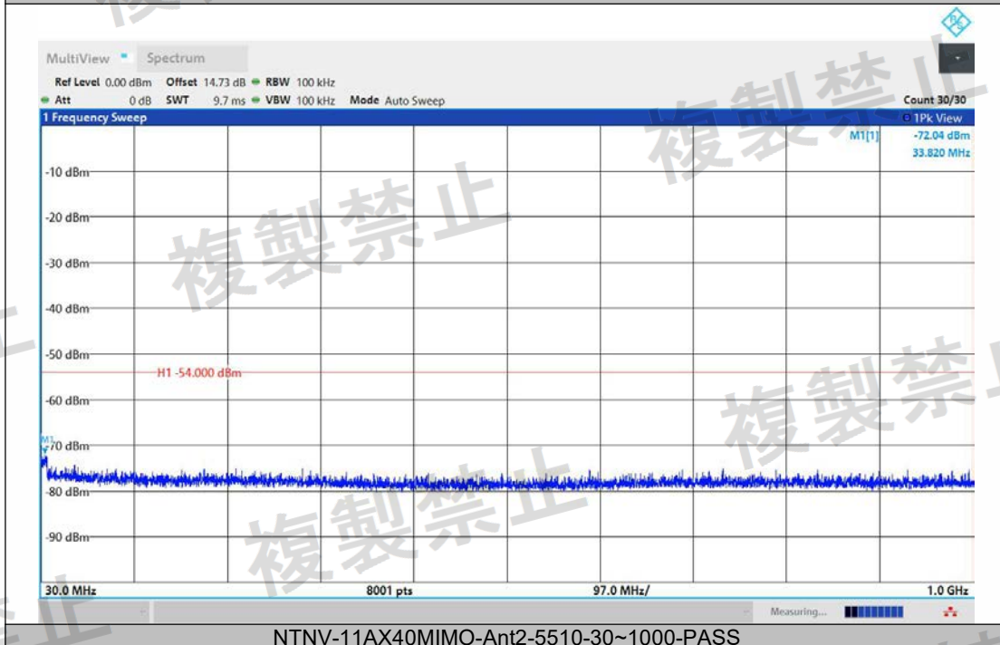
NTNV-11AX40MIMO-Ant2-5510-30~1000-PASS
