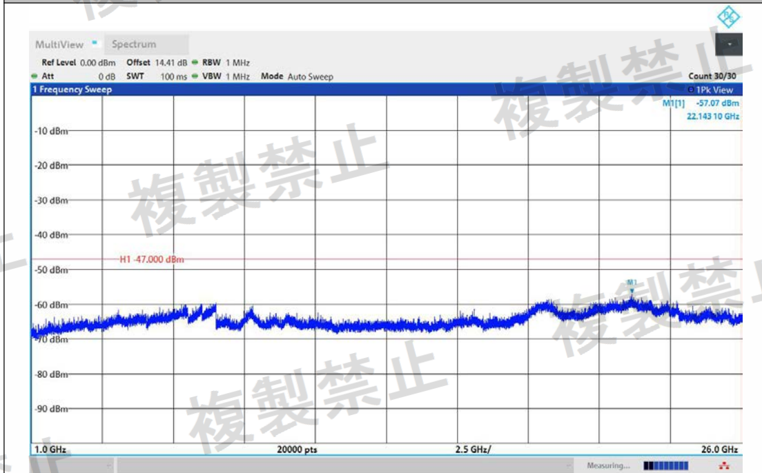
NTNV-11AC20MIMO-Ant2-5700-1000~26000-PASS
