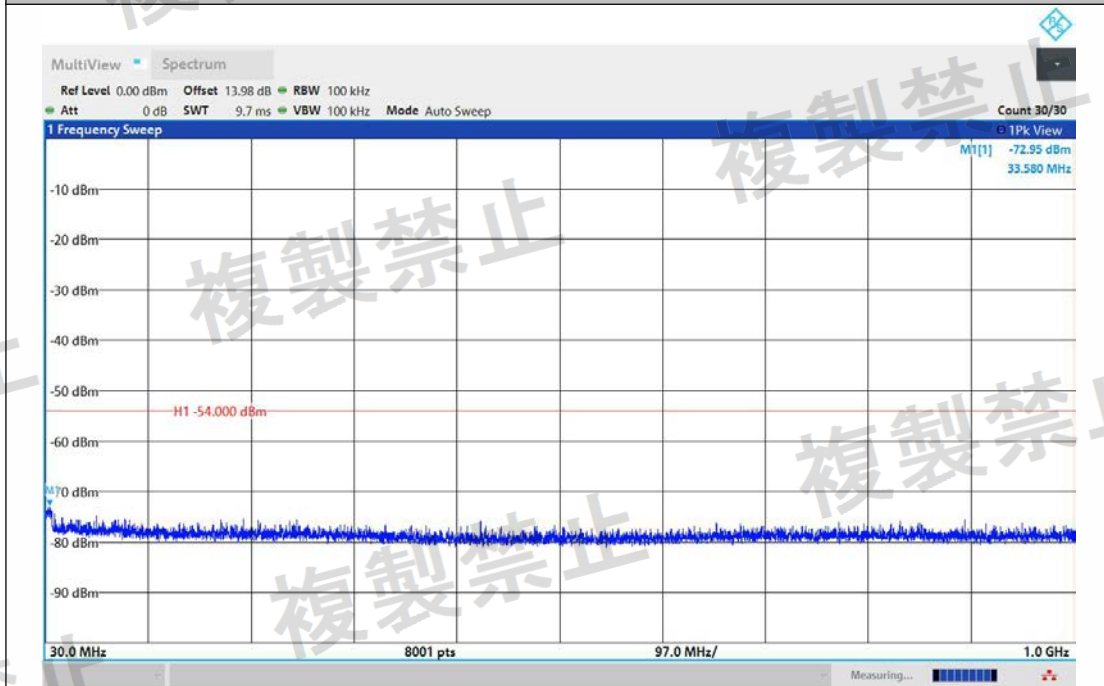
NTNV-11AX40MIMO-Ant2-5190-30~1000-PASS
