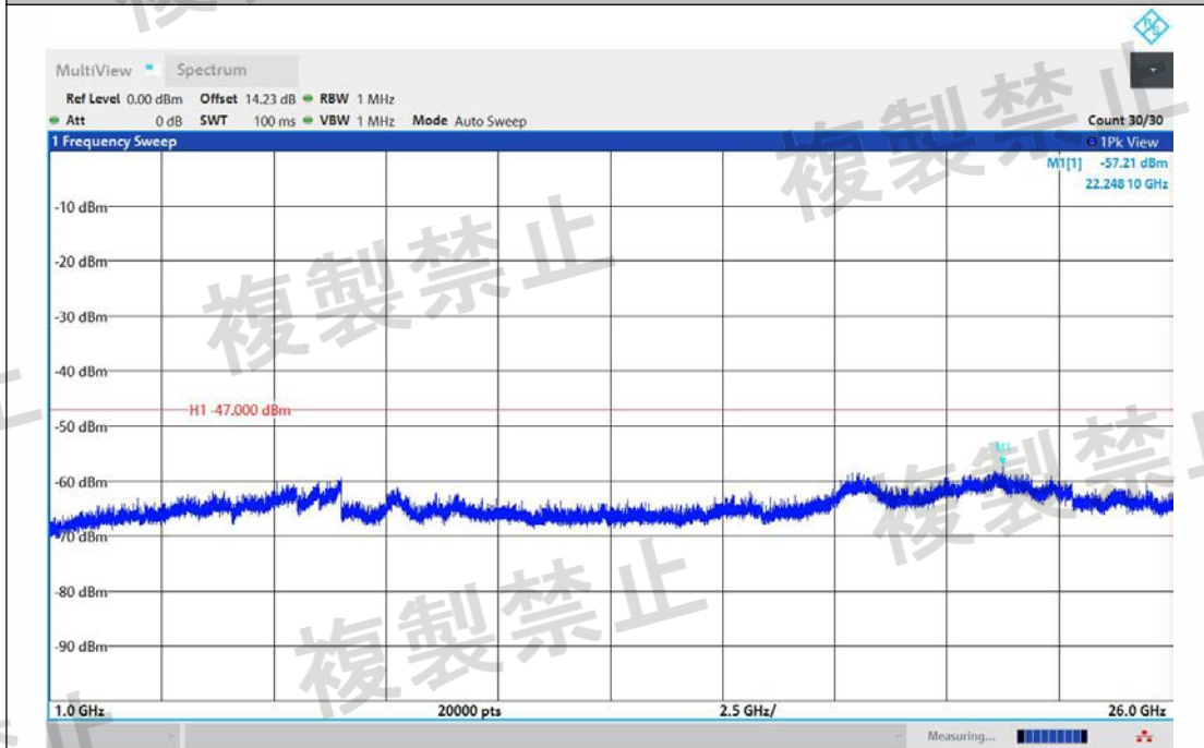
NTNV-11AX20MIMO-Ant2-5580-1000~26000-PASS
