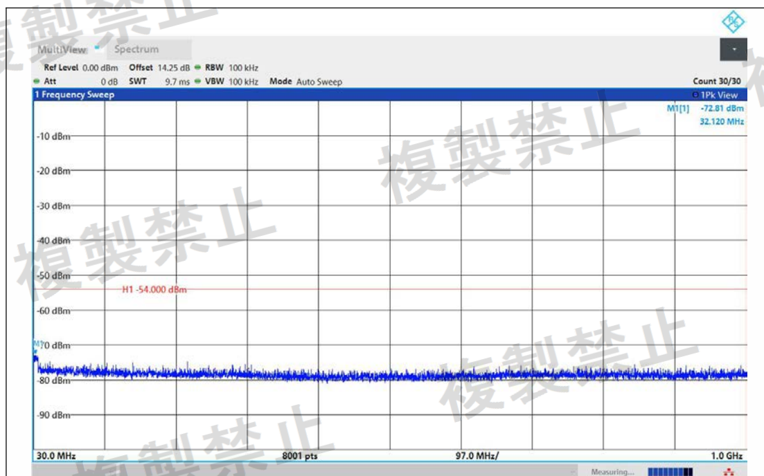
NTVN-11AX20MIMO-Ant1-5280-30~1000-PASS
