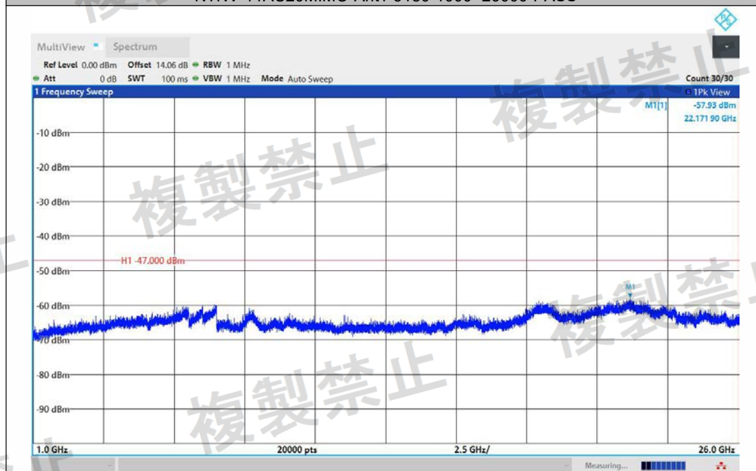
NTNV-11AC20MIMO-Ant2-5180-1000~26000-PASS
