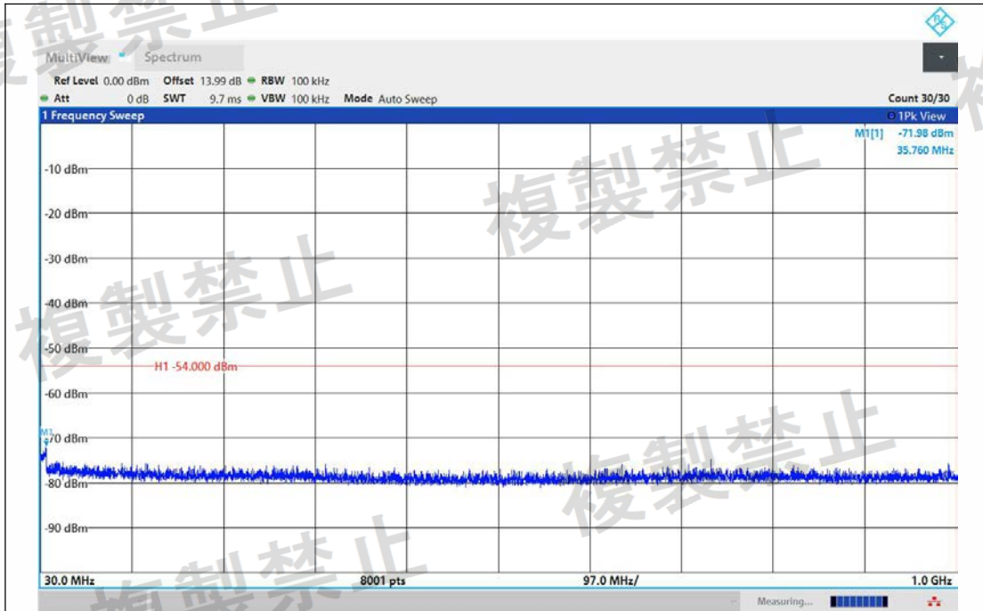
NTVN-11AC40MIMO-Ant1-5230-30~1000-PASS
