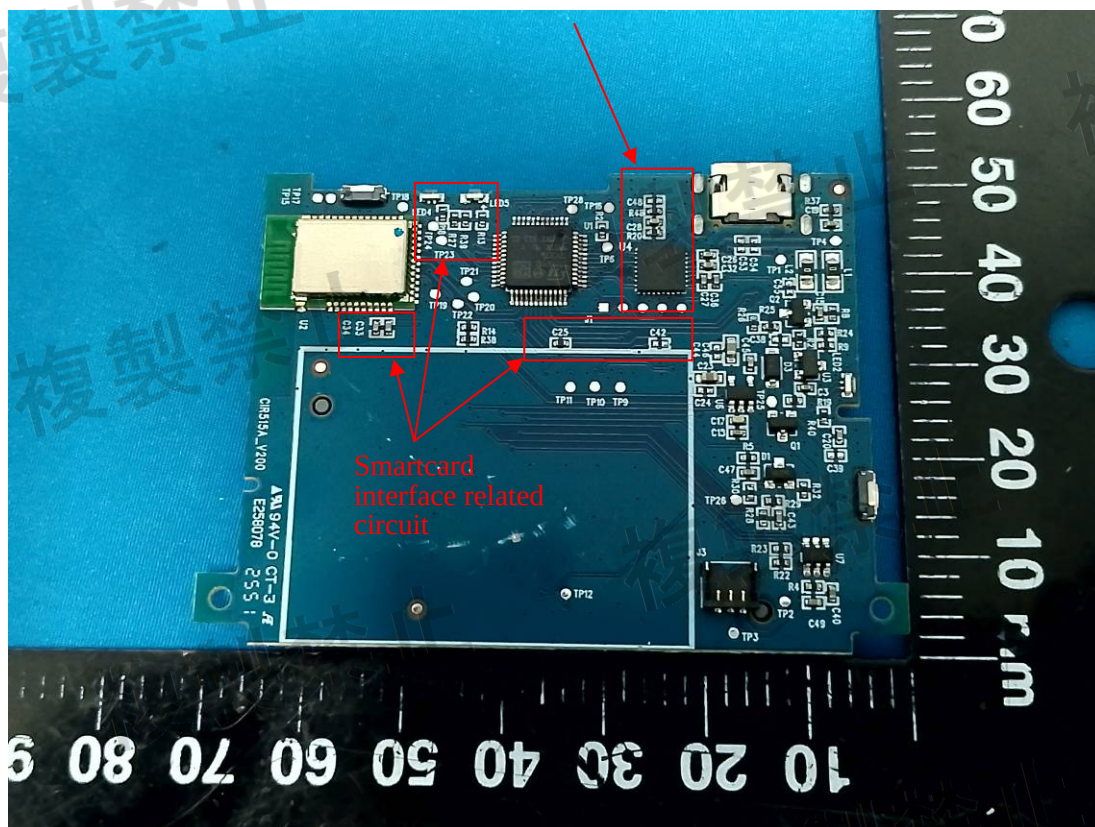
Smartcard interface IC & related circuit
