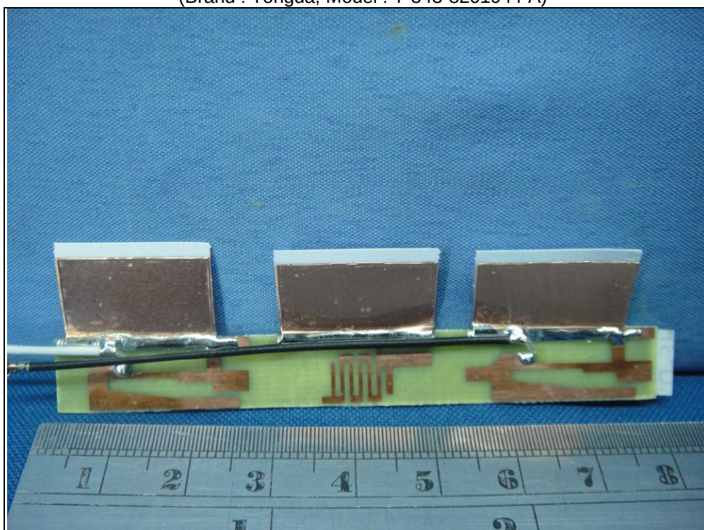
Antenna set 2 – (Brand : Tongda, Model : T-543-8201044-A)
