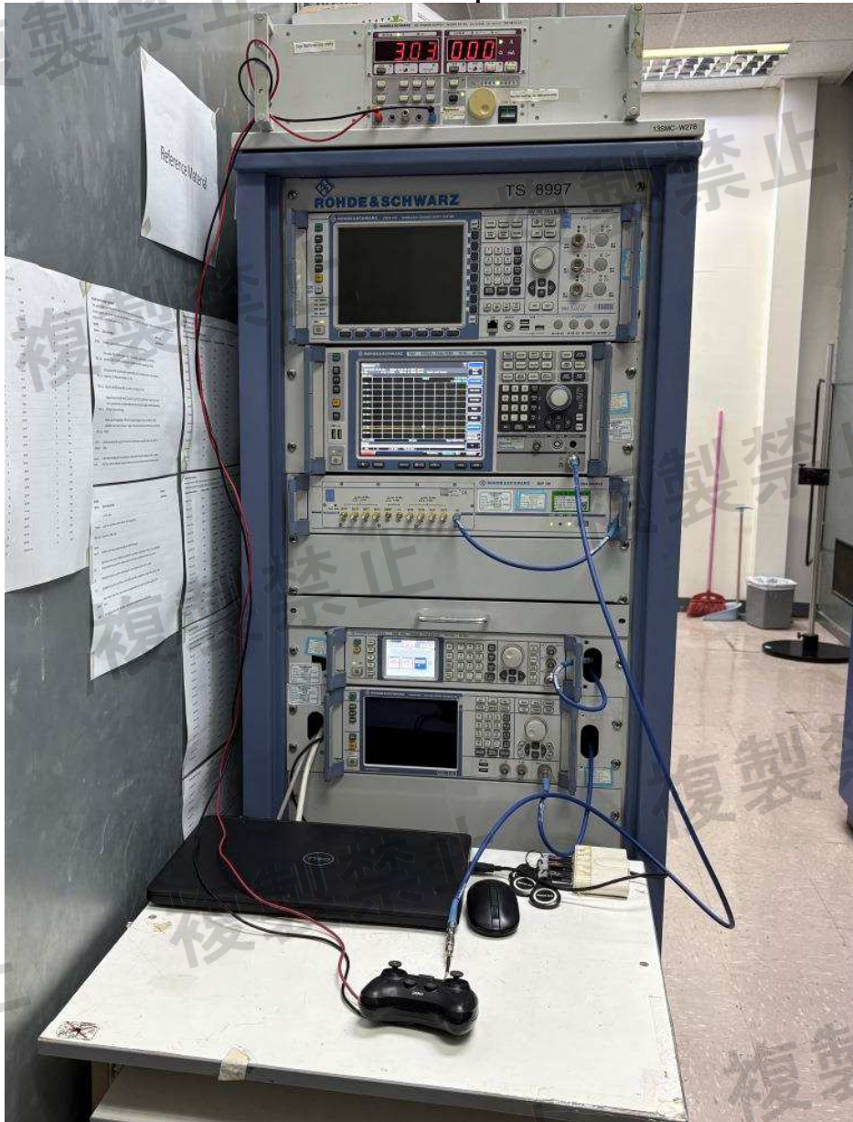
Test Setup
