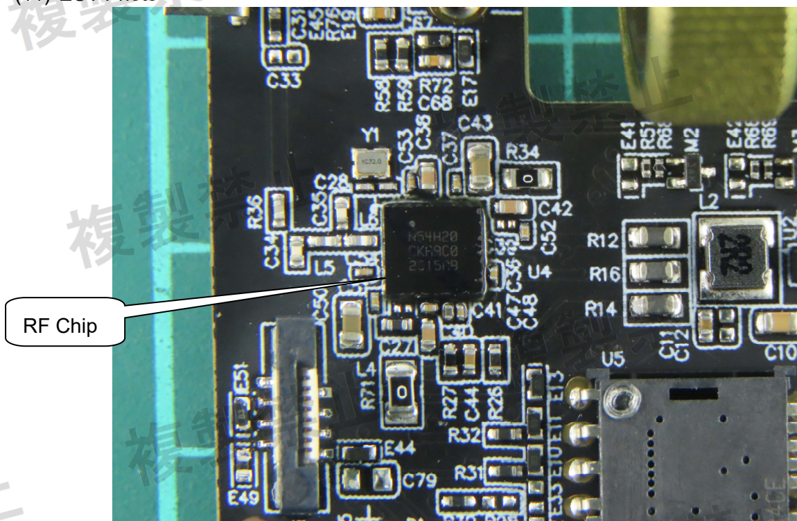
(11) EUT Photo
