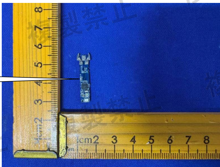
Chip ANT
