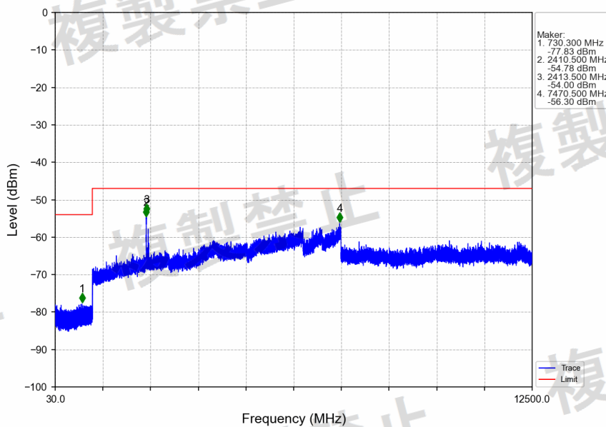
GFSK_DH5_2441MHz_Ant1_NTNV
