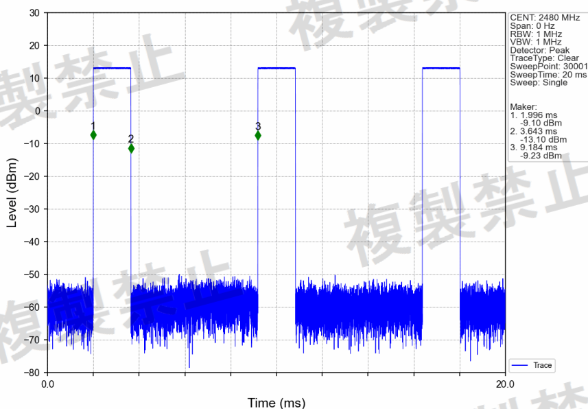
GFSK_DH5_2480MHz_Ant1_NTNV
