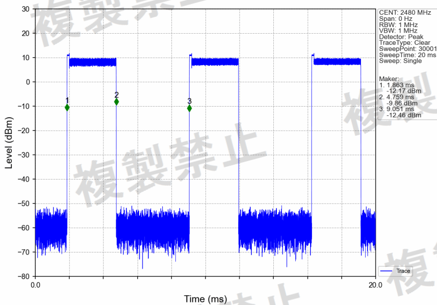
Pi/4DQPSK_2DH5_2480MHz_Ant1_NTNV
