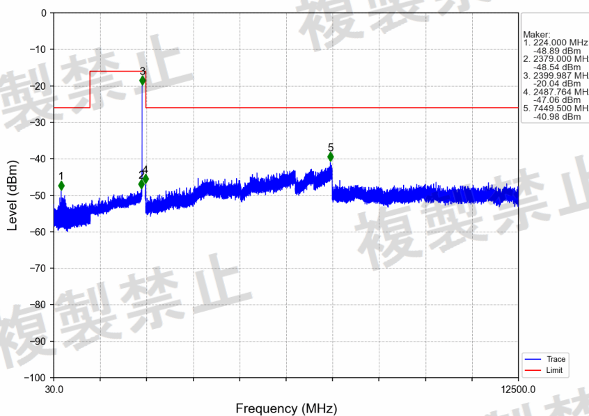
Pi/4DQPSK_2DH5_2402MHz_Ant1_NTNV
