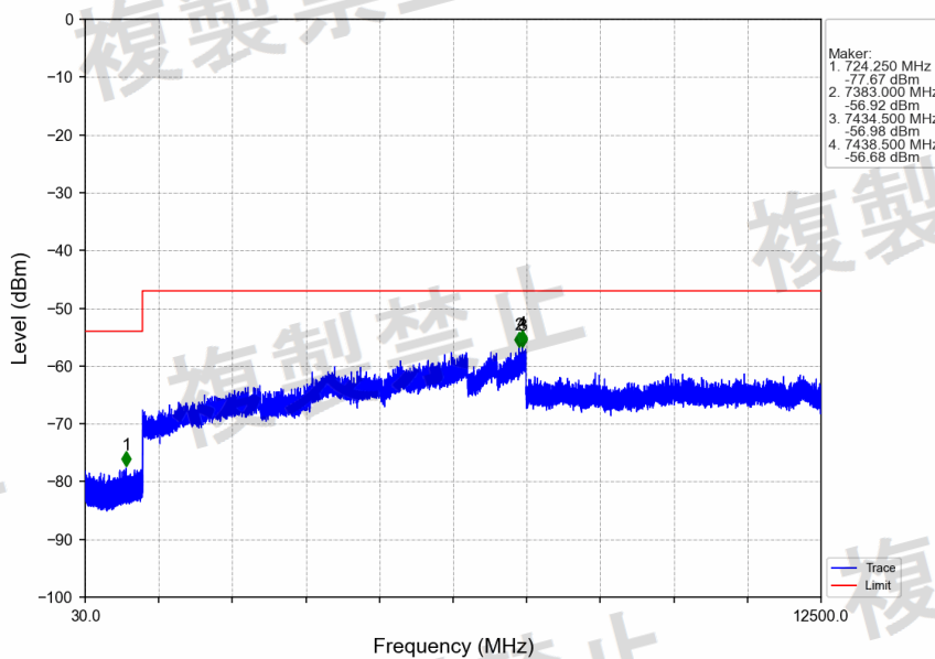
8DPSK_3DH5_2441MHz_Ant1_NTNV
