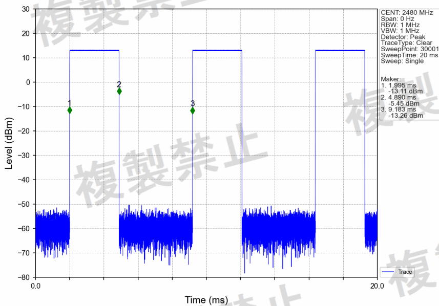
GFSK_DH5_2480MHz_Ant1_NTNV
