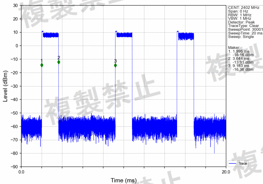
8DPSK_3DH3_2402MHz_Ant1_NTNV
