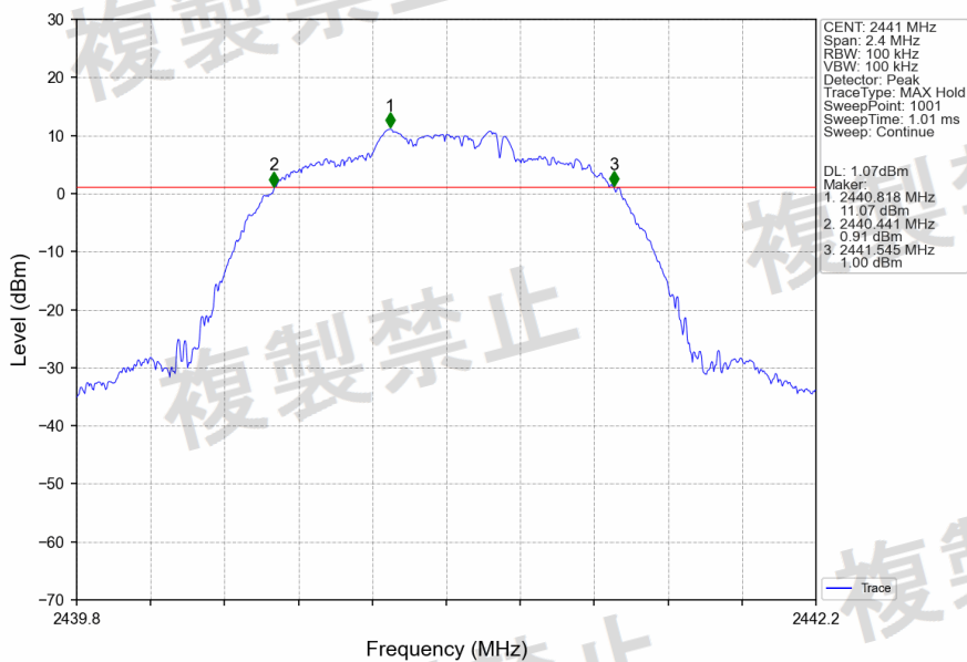
8DPSK_3DH5_2441MHz_Ant1_NTNV
