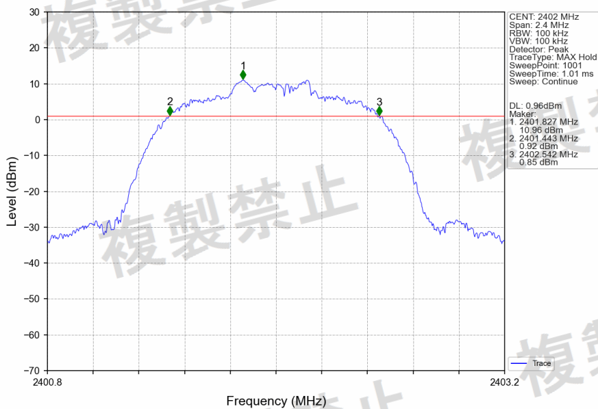
Pi/4DQPSK_2DH5_2402MHz_Ant1_NTNV
