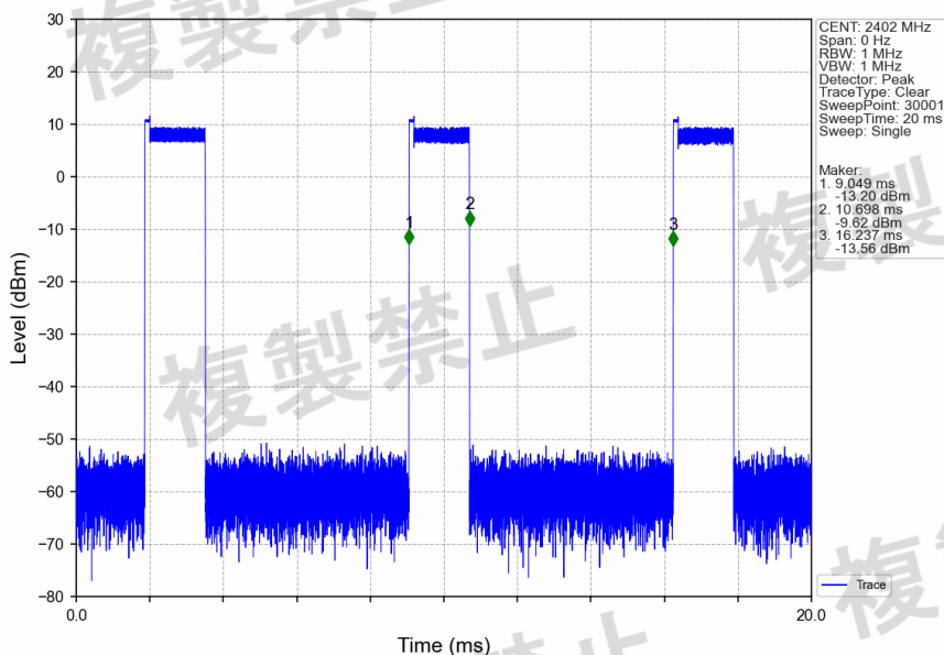
Pi/4DQPSK_2DH3_2402MHz_Ant1_NTNV
