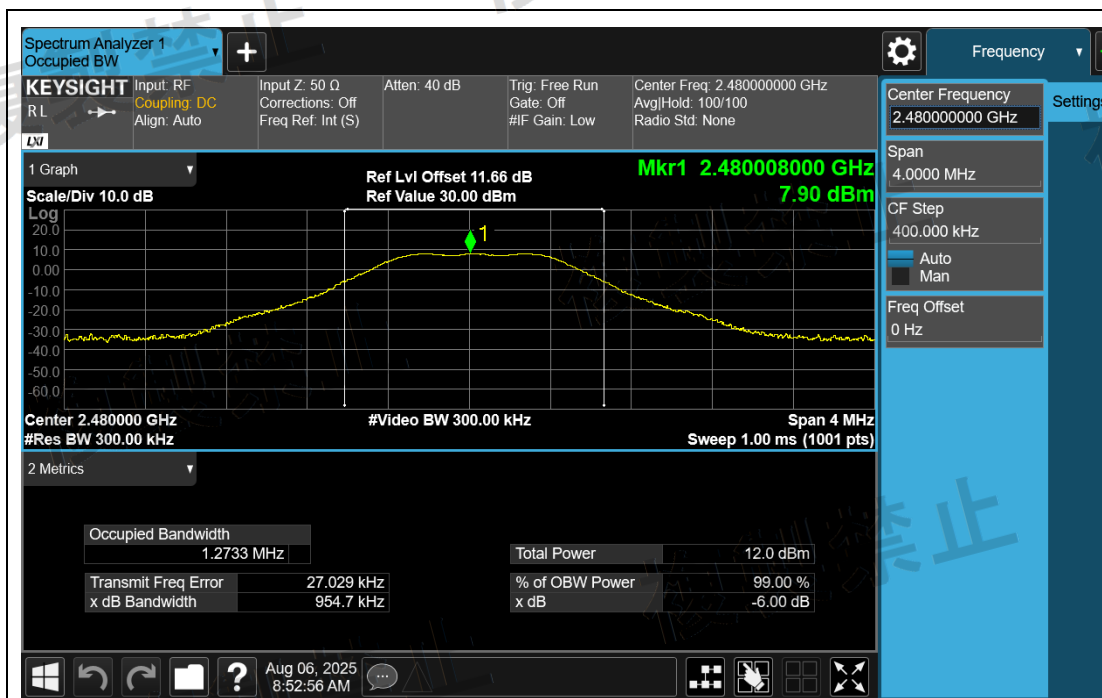
NTNV_BLE_1M_Ant1_2480
