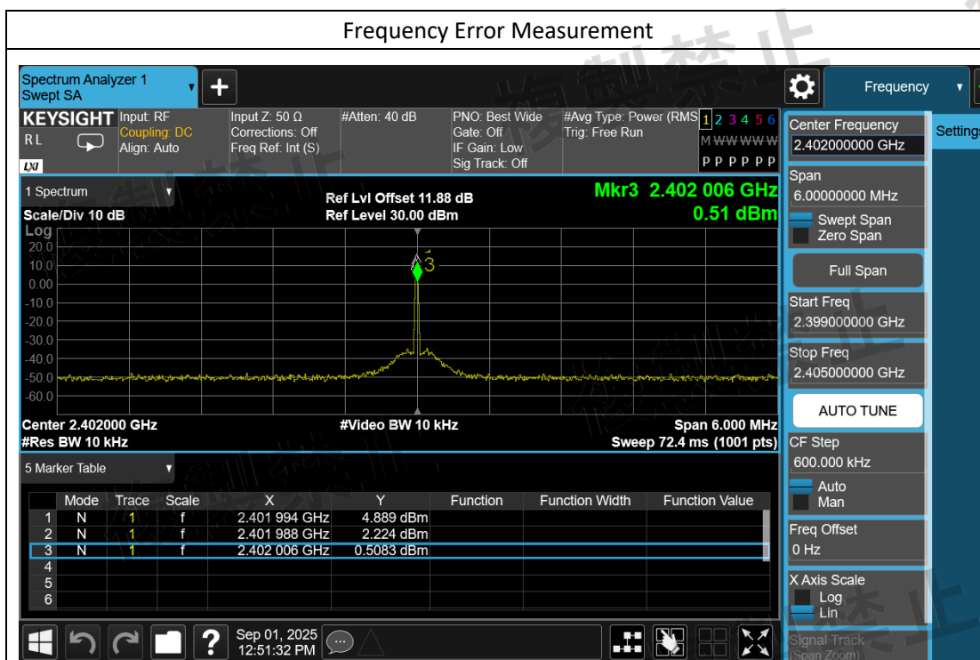
NTNV_BLE_1M_Ant1_2402
