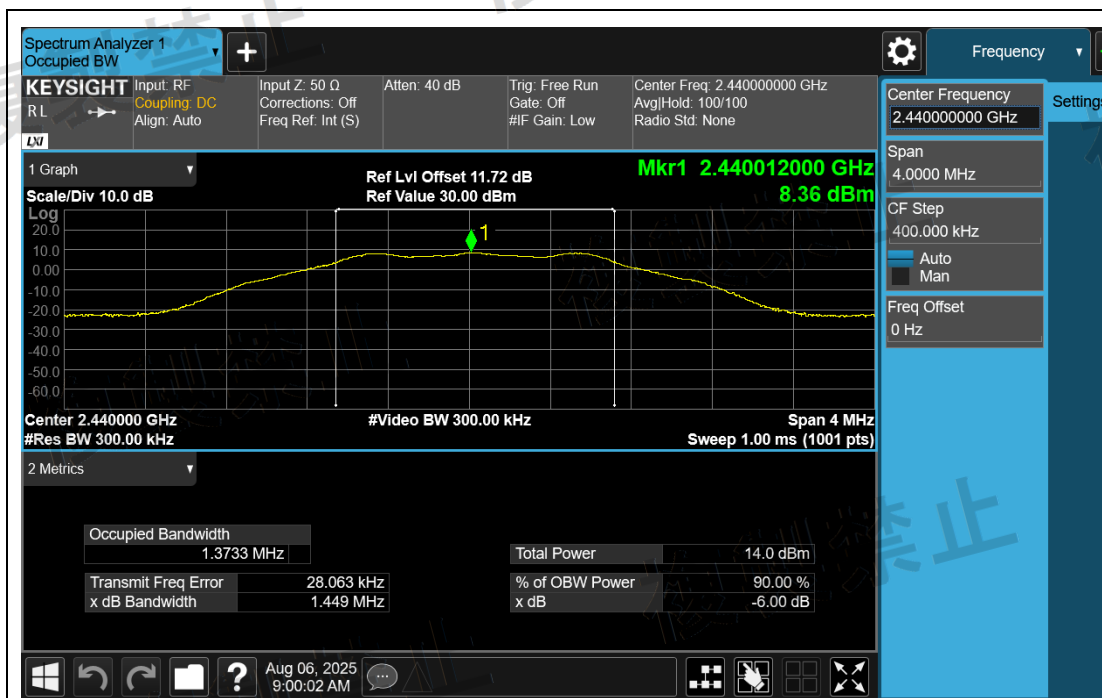
NTNV_BLE_2M_Ant1_2440
