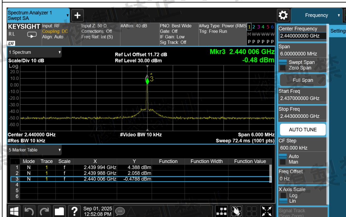
NTNV_BLE_1M_Ant1_2440
