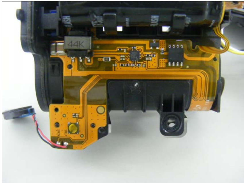
view of Keypad PCB #2
