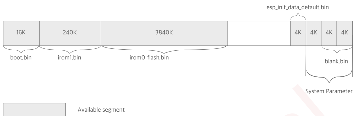
Figure 2-3. Flash Layout
